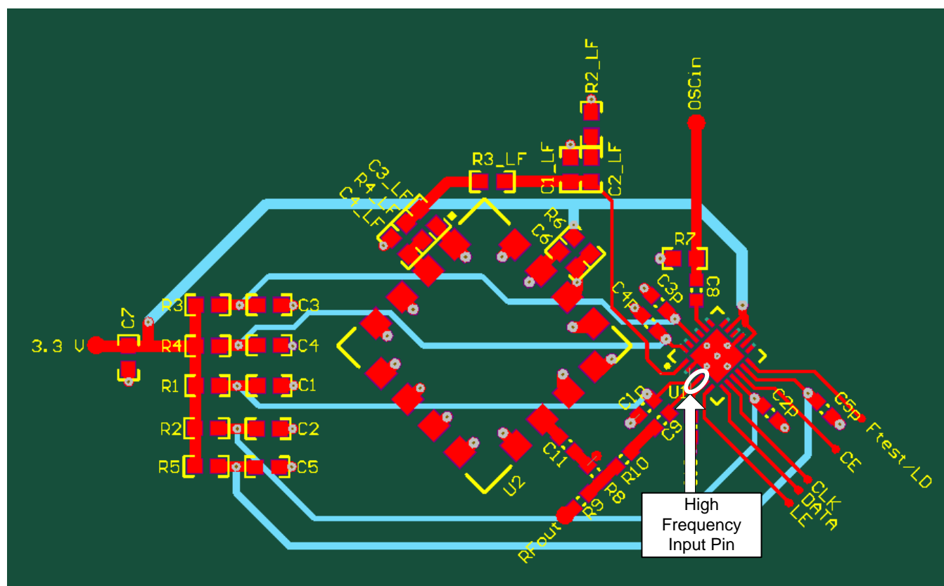
Figure 27. Layout Example
