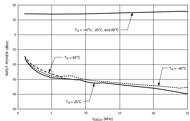
Figure 9. OSCin Sensitivity
