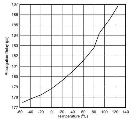
Figure 5-18. Propagation Delay
