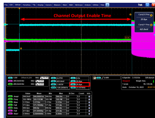
Figure 5-19. Channel Enable Setting Time
