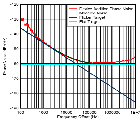
Figure 5-6. Flicker Noise
