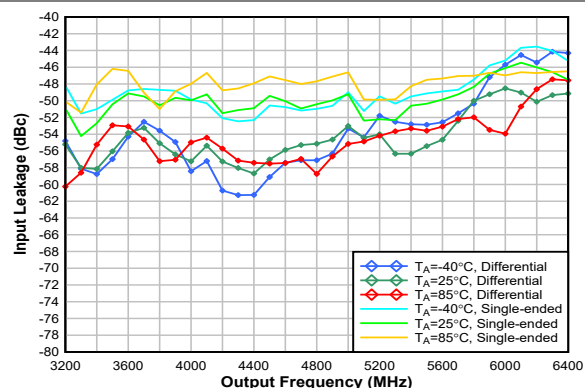
Figure 5-21. Multiplier 1/2 Sub-Harmonic in X2 Mode
