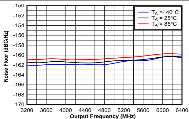
Figure 5-9. Noise Floor in x2 Multiplier Mode
