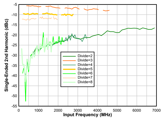
Figure 5-17. Second Harmonic in Divide Mode (Single-Ended)
