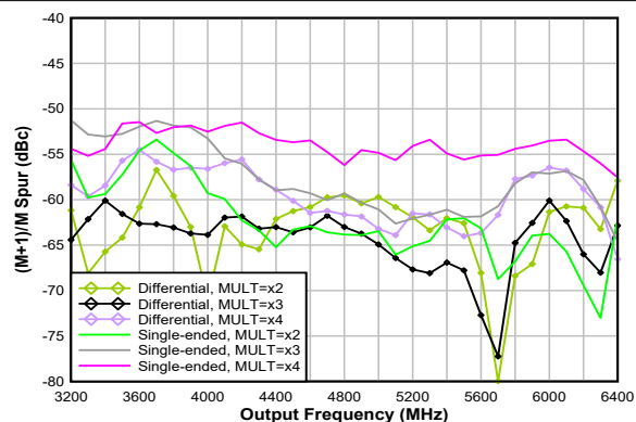
Figure 5-23. Multiplier Intermodulation (M+1)/M Spur
