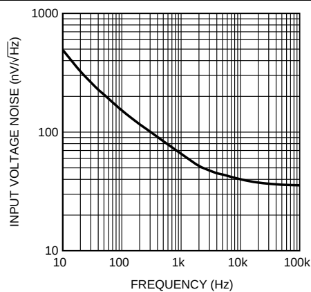
Figure 12. Input Voltage Noise vs Frequency
