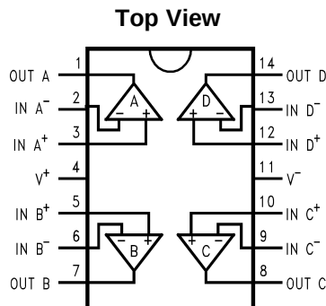
Figure 4. 14-Pin TSSOP Package See Package Number PW0014A
