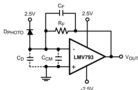
Figure 56. Transimpedance Amplifier
