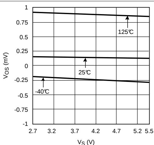
Figure 6. V_{OS} vs Supply Voltage
