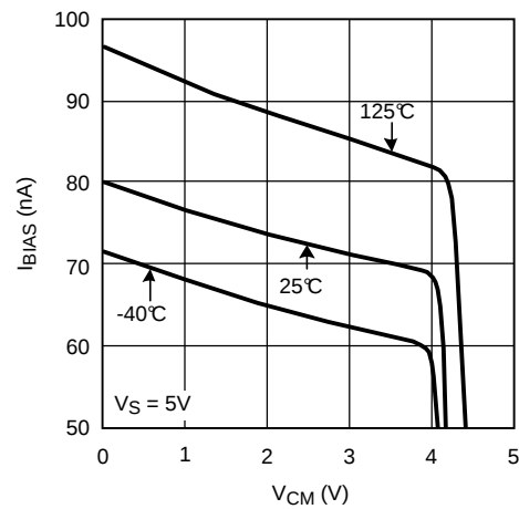
Figure 8. I_{BIAS} vs V_{CM}
