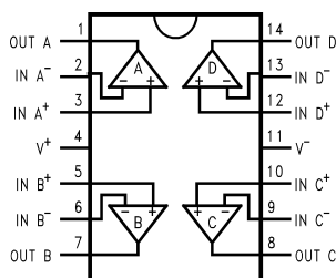
Pin Functions: LMV651
