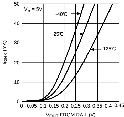
Figure 16. Sinking Current vs Output Voltage (LMV652)
