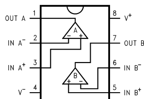
LMV652 DGK Package 8-Pin VSSOP Top View
