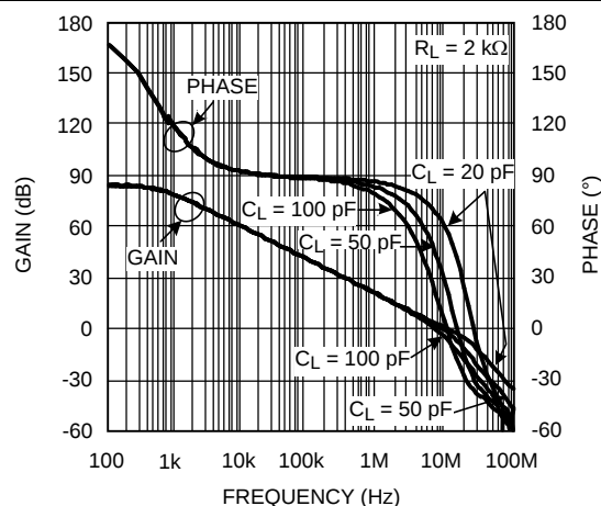
Figure 18. Open-Loop Gain and Phase With Capacitive Load
