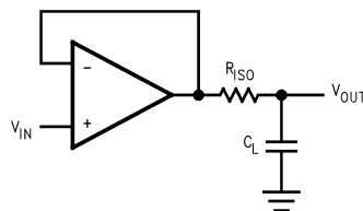
Figure 36. Compensation by Isolation Resistor
