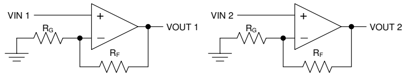
Figure 7-7. Schematic Representation
