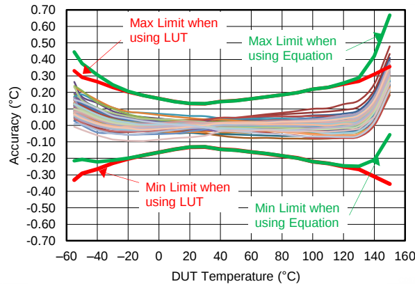
Figure 28. LMT70 Performance Using LUT and Linear Interpolation
