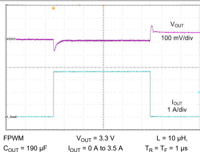
Figure 9-28. Load Transient
