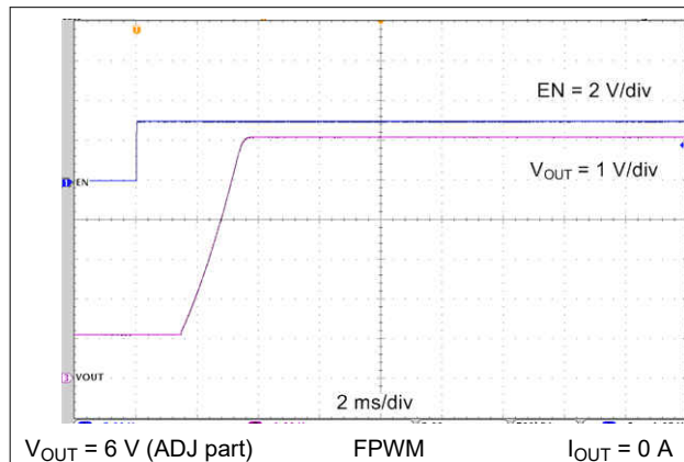
Figure 9-31. Start-Up Waveform
