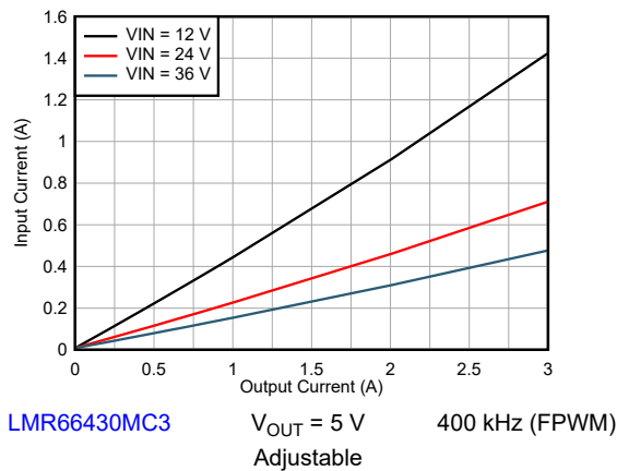
Figure 8-22. Input Current vs Load Current
