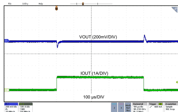
LMR66430MC3 V_{OUT} = 3.3 V 2.2 MHz (FPWM) 0 A to 1 A, 1 A / \mu s Fixed
