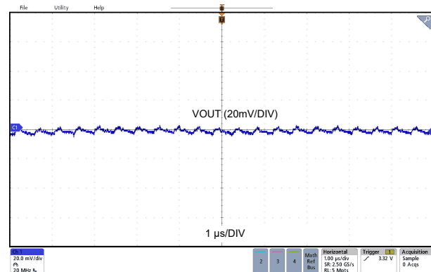
LMR66430MC3 V_{OUT} = 3.3 V 2 A Load Fixed
