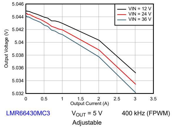
Figure 8-21. Line and Load Regulation
