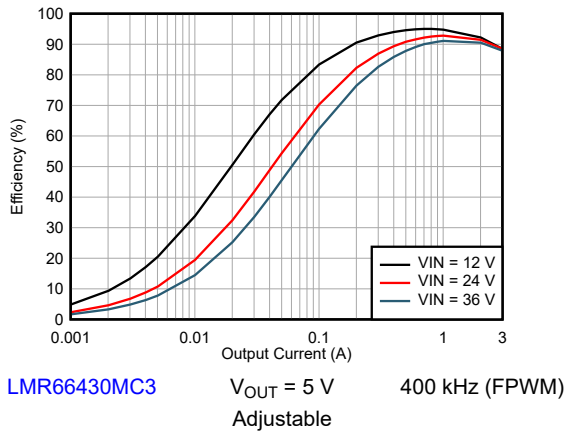
Figure 8-20. Efficiency
