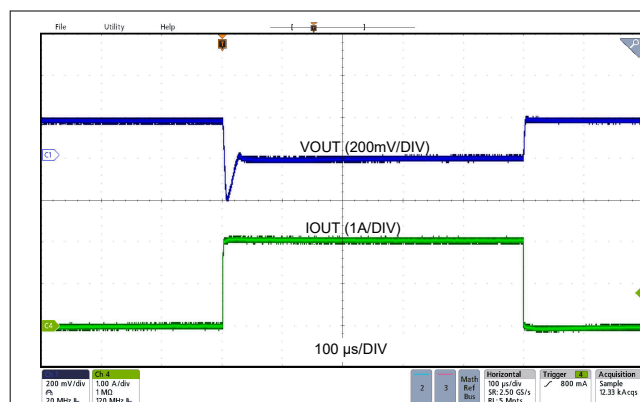
LMR66430MC3 V_{OUT} = 3.3 V 2.2 MHz (Auto) 0 A to 2 A, 1 A / \mu s Fixed
