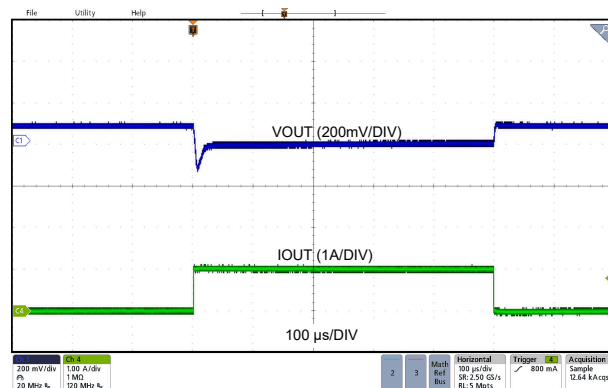
LMR66430MC3 V_{OUT} = 3.3 V 2.2 MHz (Auto) 0 A to 1 A, 1 A / \mu s Fixed
