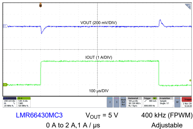
Figure 8-24. Load Transient
