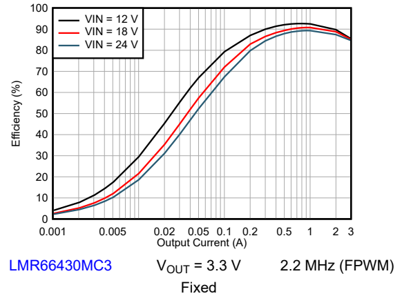
Figure 8-5. Efficiency
