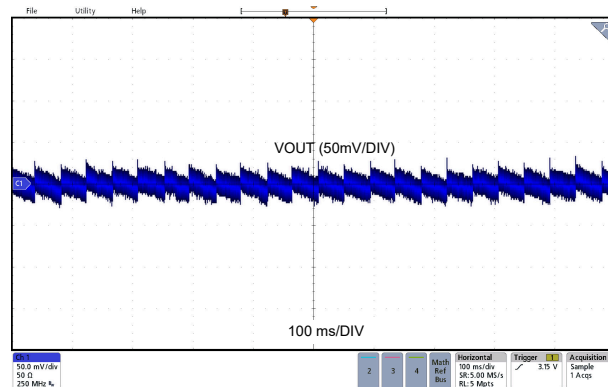
LMR66430MC3 V_{OUT} = 3.3 V No Load Fixed
