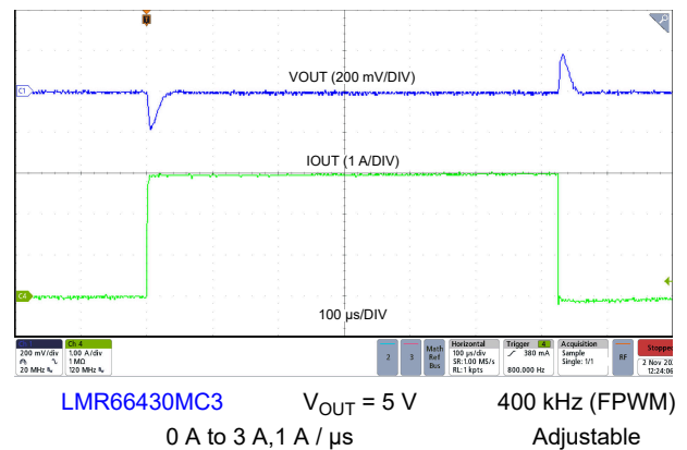
Figure 8-23. Load Transient
