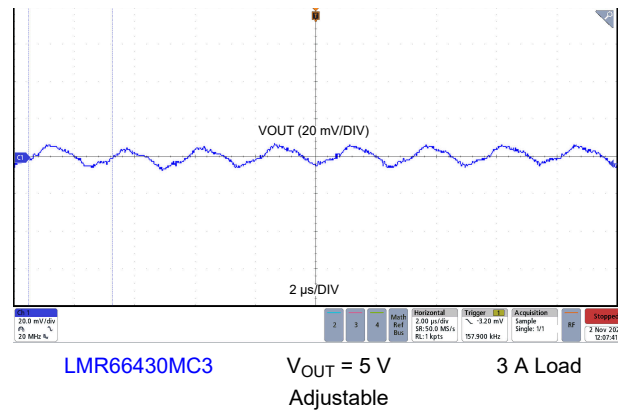
Figure 8-25. Output Voltage Ripple
