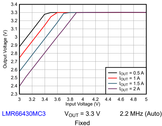
Figure 8-6. Dropout
