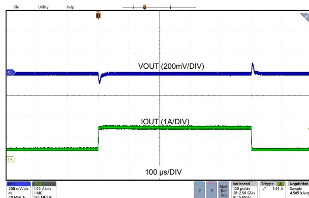
LMR66430MC3 V_{OUT} = 3.3 V 2.2 MHz (Auto) 0.5 A to 1.5 A, 1 A / \mu s Fixed
