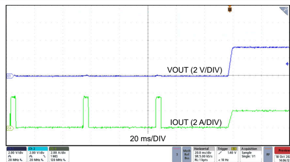
Figure 7-15. Hiccup Exit
