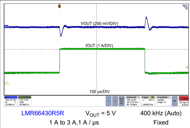
Figure 8-9. Load Transient
