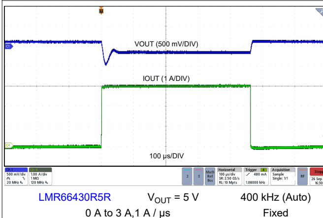
Figure 8-8. Load Transient
