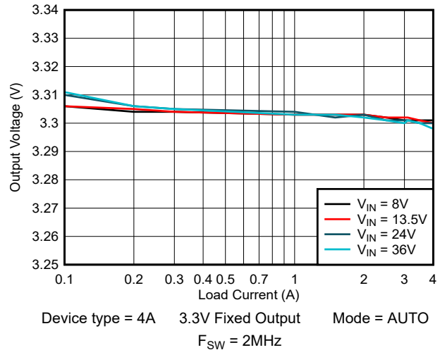
Figure 8-3. Load Regulation
