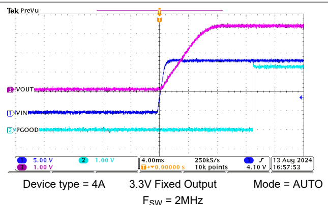
Figure 8-7. Start-Up Operation
