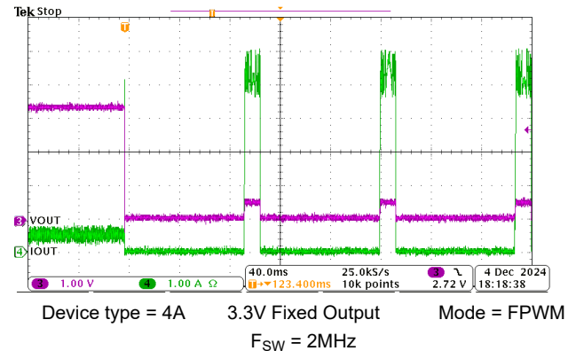
Figure 8-9. Short-Circuit Applied
