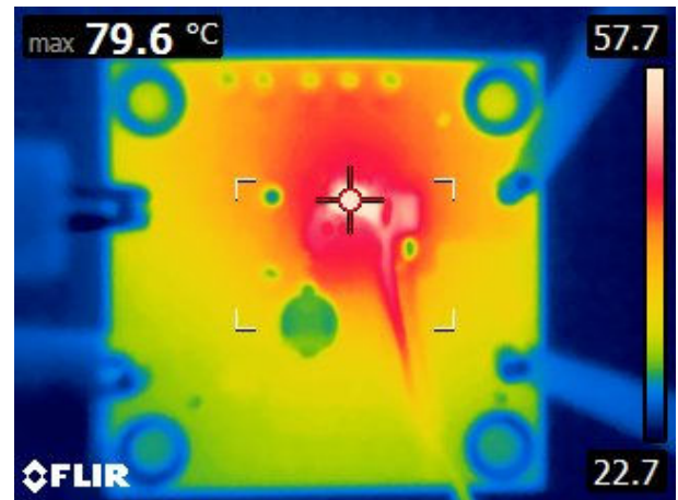
Figure 8-9. Short-Circuit Applied
