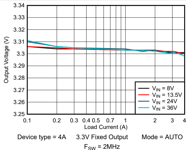
Figure 8-3. Load Regulation
