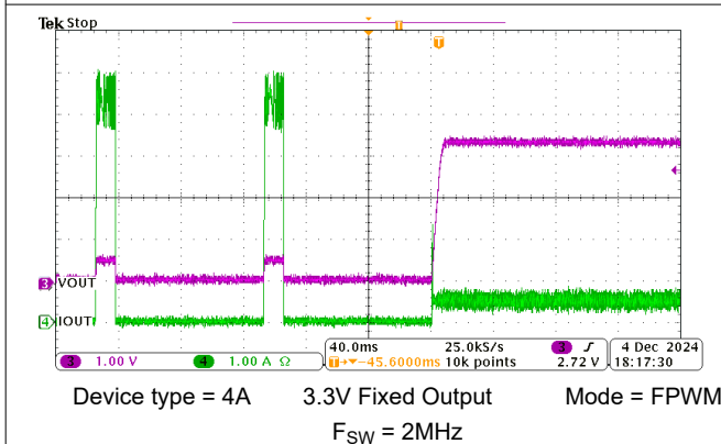
Figure 8-10. Short-Circuit Recovery
