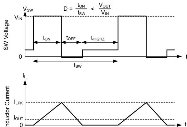
Figure 7-7. PFM Operation
