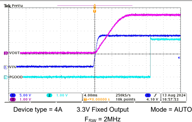
Figure 8-7. Start-Up Operation
