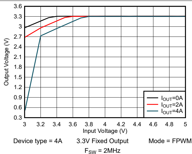
Figure 8-4. Dropout Voltage
