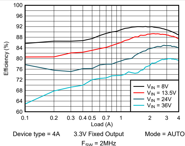
Figure 8-2. Efficiency
