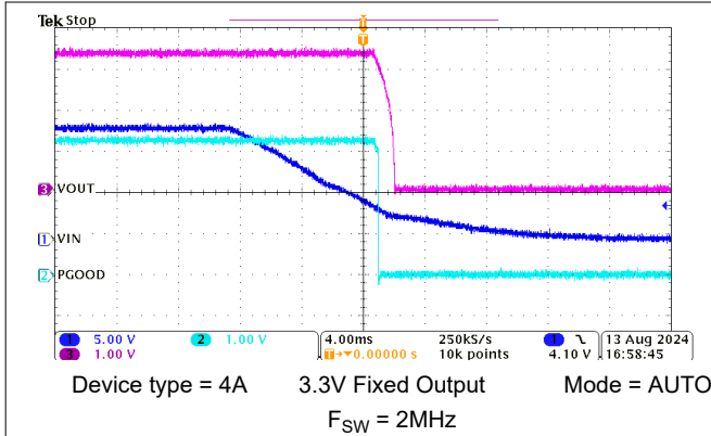
Figure 8-8. Shutdown Operation
