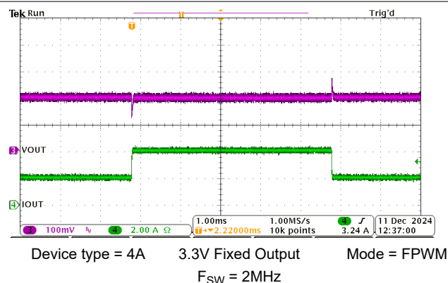
Figure 8-6. 2A to 4A Load Transient
