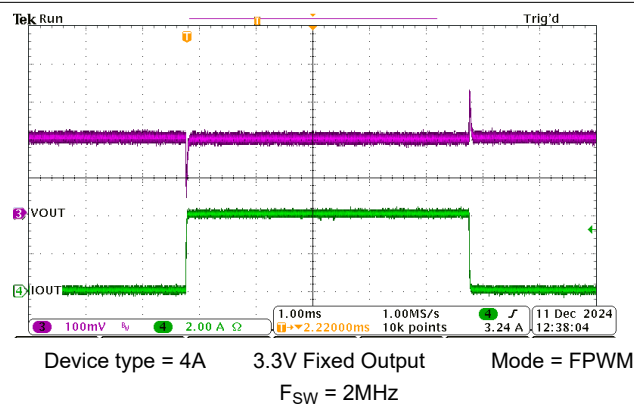
Figure 8-5. 20mA to 4A Load Transient
