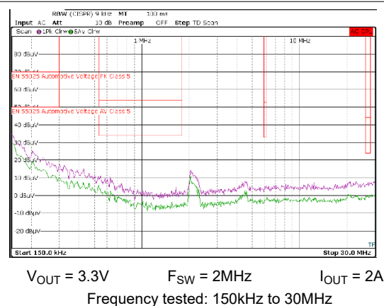
Figure 8-19. Conducted EMI versus CISPR25 Limits (Purple: Peak Signal, Green: Average Signal), LMR60440QEVm
