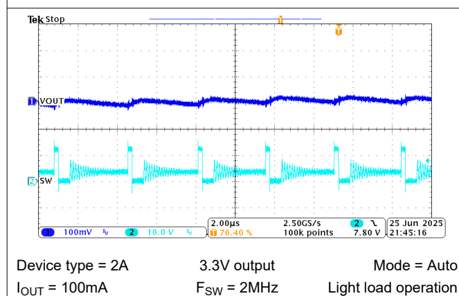
Figure 8-16. Steady State Waveform
