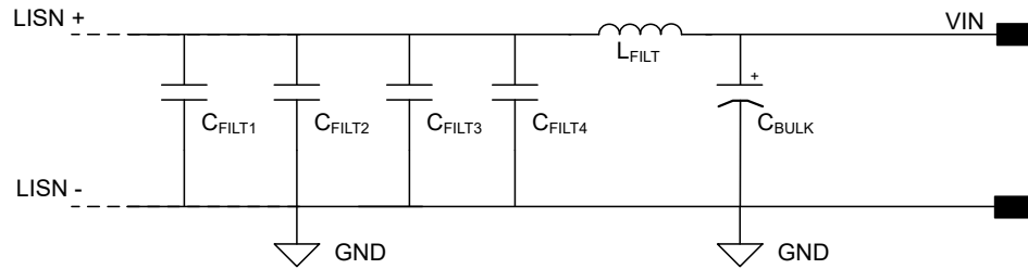
Figure 8-21. Typical Input EMI Filter Schematic
