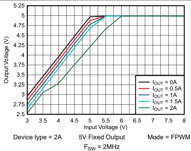
Figure 8-4. Dropout Voltage
