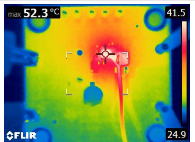
Figure 8-9. Short-Circuit Applied
