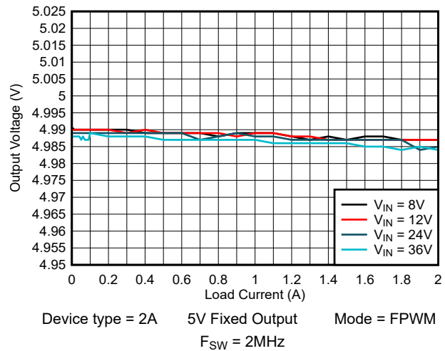
Figure 8-3. Load Regulation
