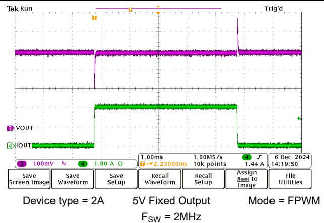
Figure 8-5. 0A to 2A Load Transient
