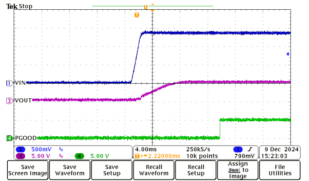
Figure 8-7. Start-Up Operation
