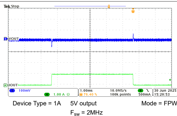
Figure 8-18. 0A to 1A Load Transient
