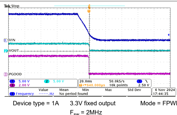
Figure 8-6. Shutdown
