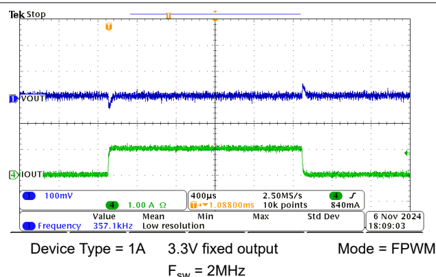
Figure 8-7. 0A to 1A Load Transient
