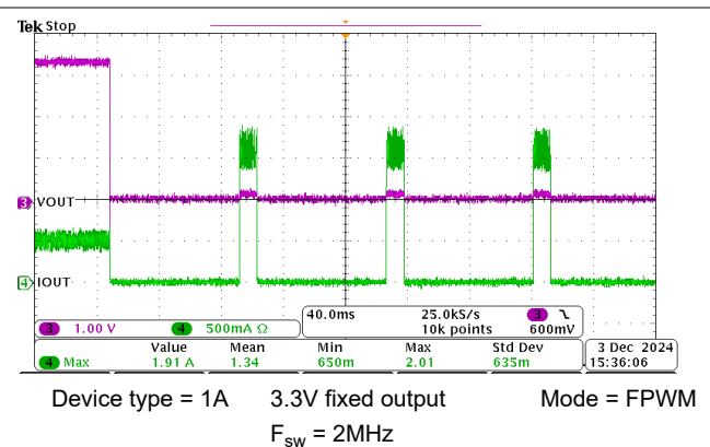
Figure 8-9. Short-Circuit Applied
