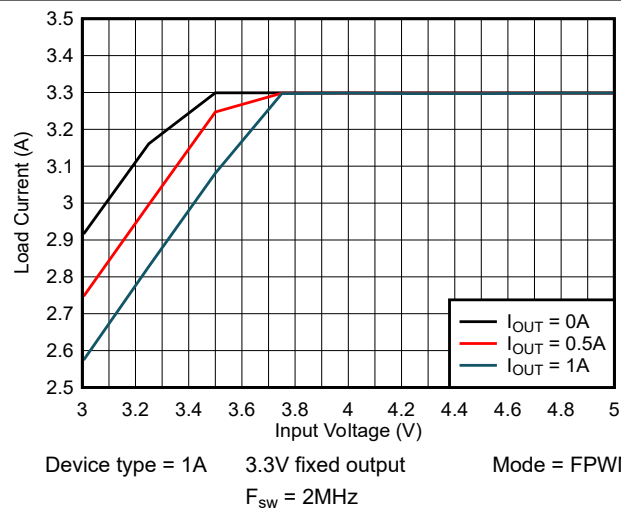
Figure 8-4. Dropout Voltage
