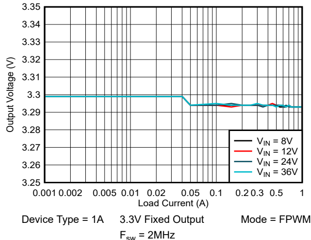
Figure 8-3. Load Regulation
