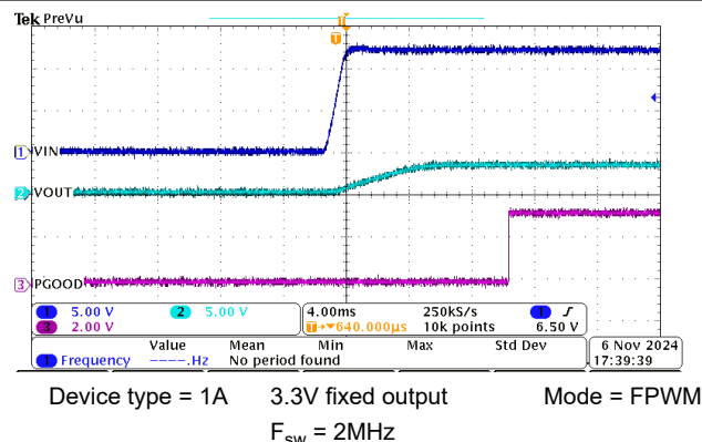
Figure 8-5. Start-up
