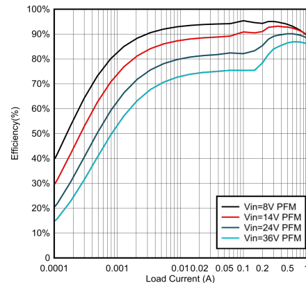
Efficiency Versus Output Current; V_{OUT} = 5V, 1100\text{kHz}
