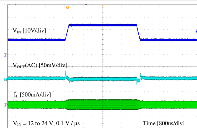
Figure 8-8. Line Transient
