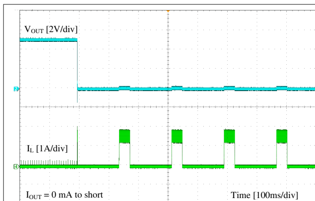
Figure 8-9. Short Protection
