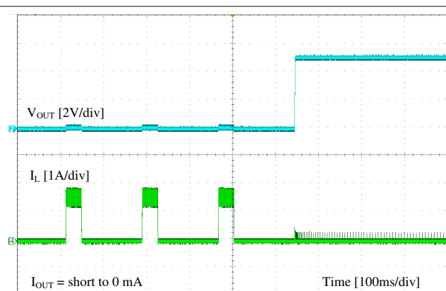
Figure 8-10. Short Recovery
