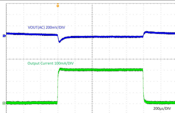
Figure 8-8. Load Transient (0mA – 300mA)
