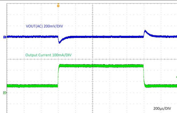
Figure 8-7. Load Transient (60mA – 240mA)
