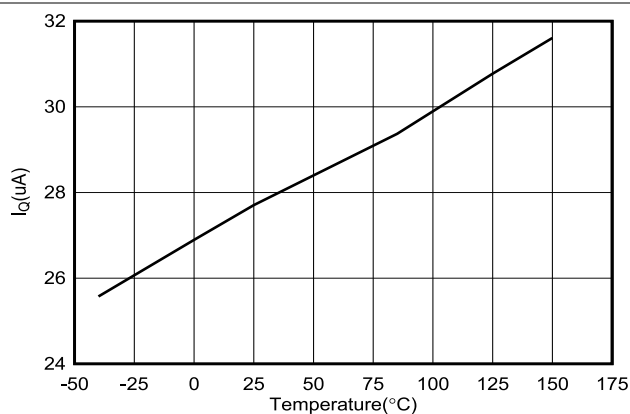
Figure 6-7. V_{IN} Quiescent Current Versus Temperature
