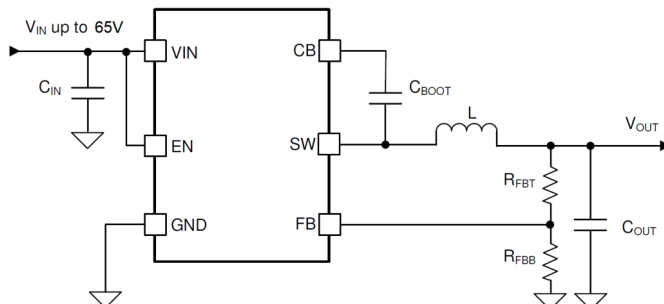
Simplified Schematic
