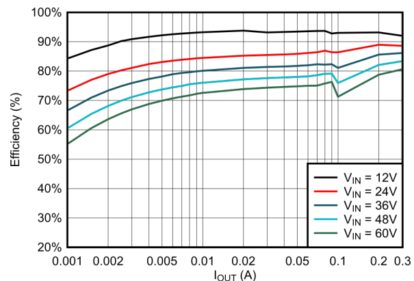
Efficiency Versus Output Current V_{OUT} = 5V, 400kHz
