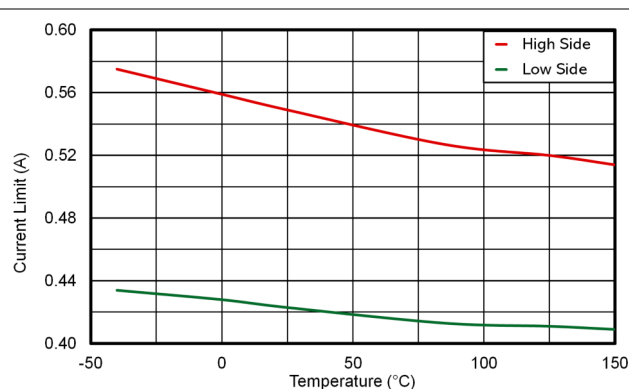
Figure 6-14. HS and LS Current Limit vs Temperature
