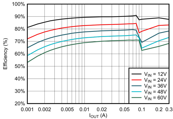
Figure 6-1. 5V PFM Efficiency vs Load Current
