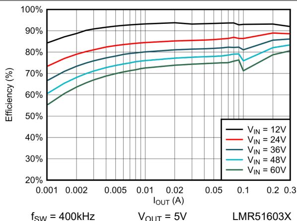
Figure 6-7. 5V PFM Efficiency vs Load Current
