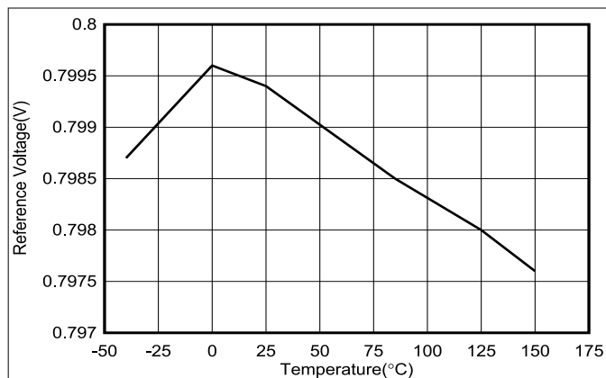
Figure 6-13. Reference Voltage vs Temperature
