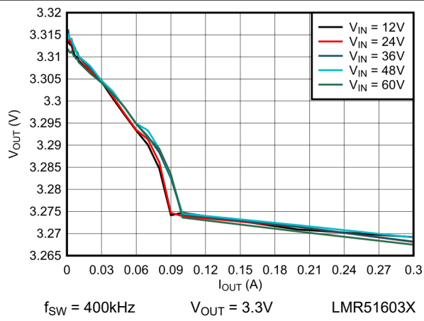
Figure 6-10. 3.3V Load Regulation
