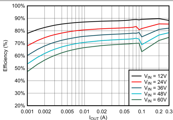
Figure 6-3. 3.3V PFM Efficiency vs Load Current
