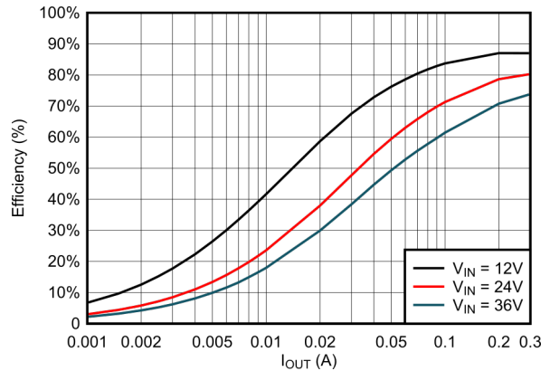
Figure 6-2. 5V FPWM Efficiency vs Load Current
