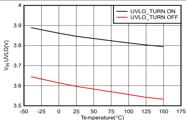
Figure 6-12. V_{IN} UVLO vs Temperature
