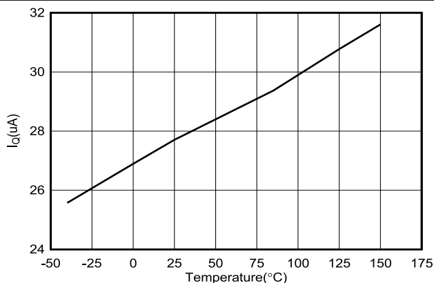
Figure 6-11. V_{IN} Quiescent Current vs Temperature
