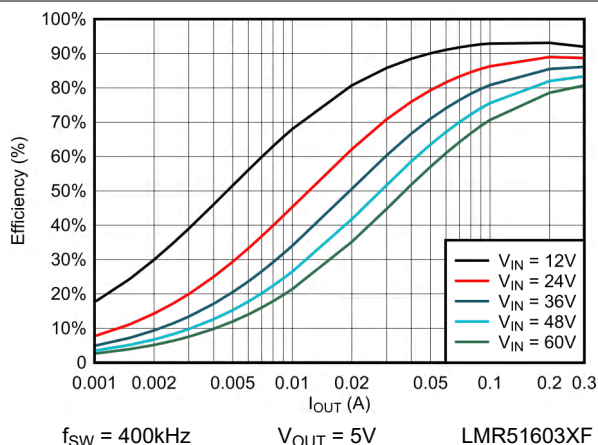
Figure 6-8. 5V FPWM Efficiency vs Load Current
