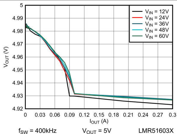
Figure 6-9. 5V Load Regulation
