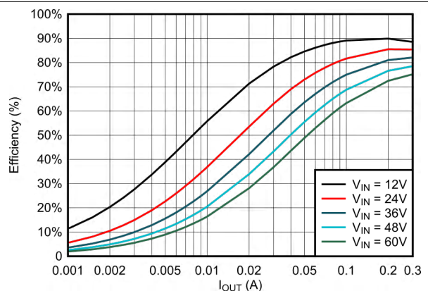
Figure 6-4. 3.3V FPWM Efficiency vs Load Current
