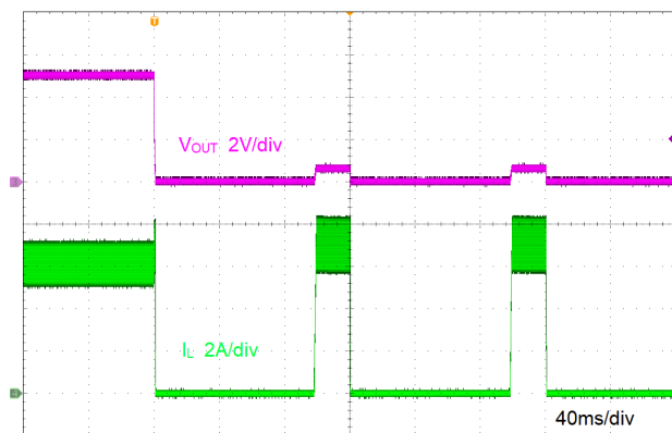
Figure 8-8. Short Protection
