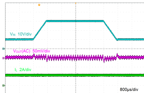
Figure 8-7. Line Transient
