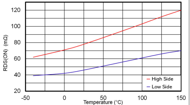
Figure 6-12. High Side and Low Side Switches R_{DS\_ON}
