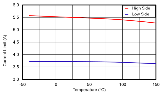
Figure 6-17. LMR51435-Q1 High Side and Low Side Current Limits
