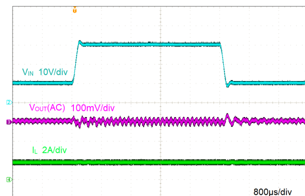
Figure 8-7. Line Transient
