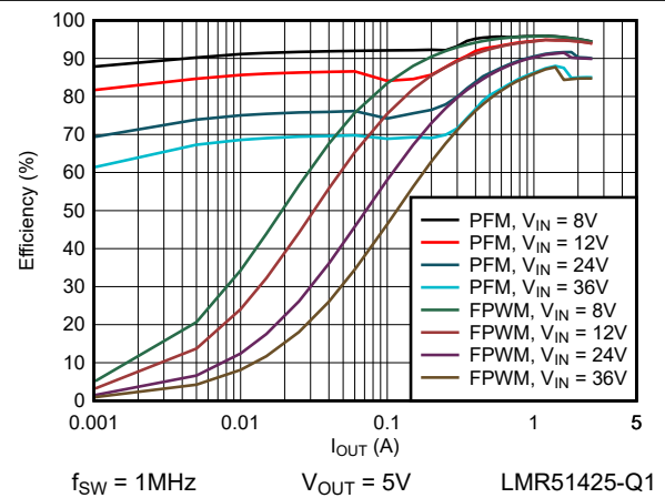
Figure 6-6. 5V Efficiency versus Load Current
