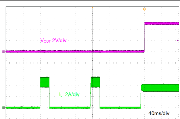
Figure 8-9. Short Recovery
