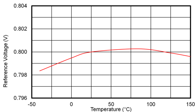
Figure 6-15. Reference Voltage
