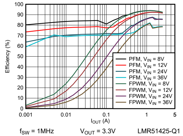
Figure 6-8. 3.3V Efficiency versus Load Current
