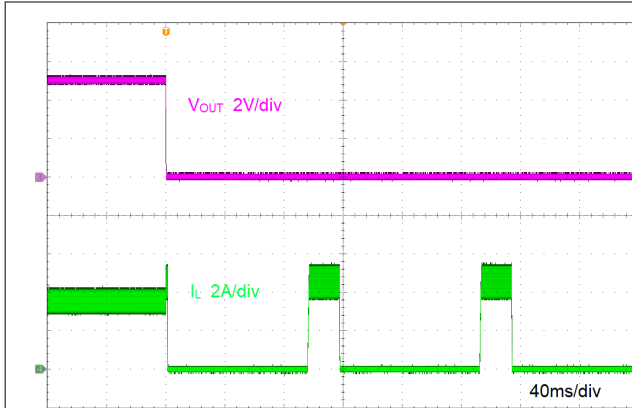
Figure 8-8. Short Protection
