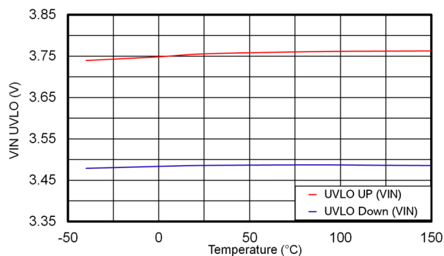
Figure 6-14. V_{IN} UVLO
