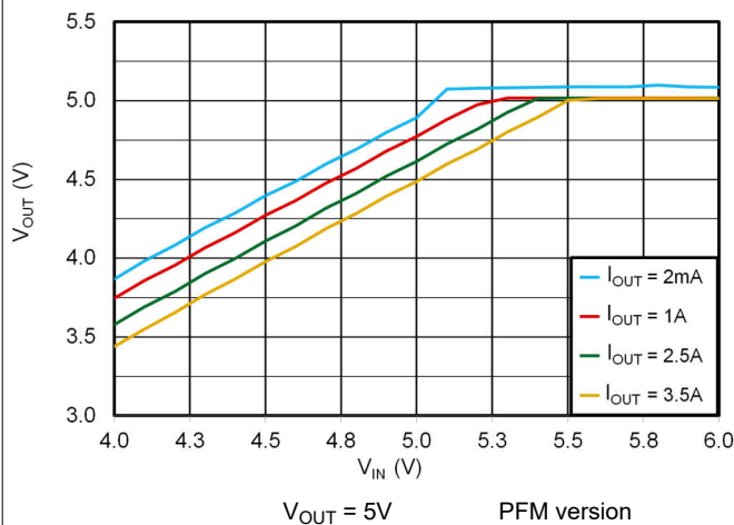
Figure 6-11. 5V Dropout
