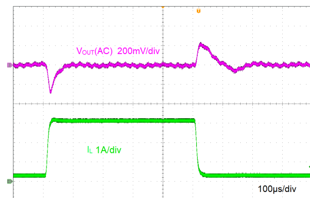
Figure 8-6. Load Transient
