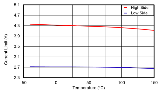
Figure 6-18. LMR51425-Q1 High Side and Low Side Current Limits
