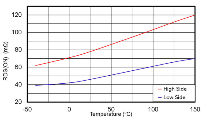
Figure 6-16. High Side and Low Side Switches R_{DS(on)}
