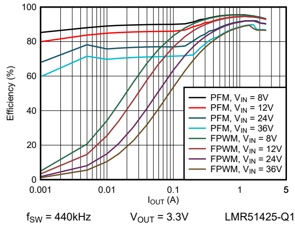
Figure 6-7. 3.3V Efficiency versus Load Current
