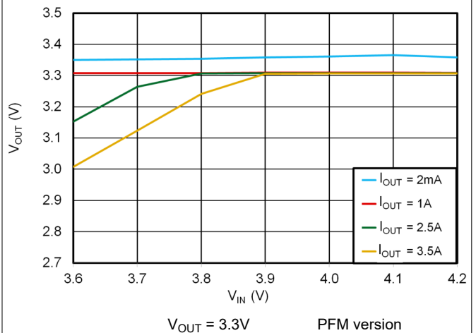
Figure 6-12. 3.3V Dropout
