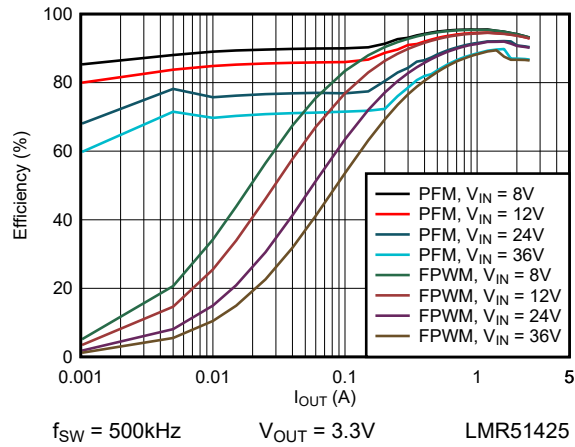
Figure 6-7. 3.3V Efficiency versus Load Current
