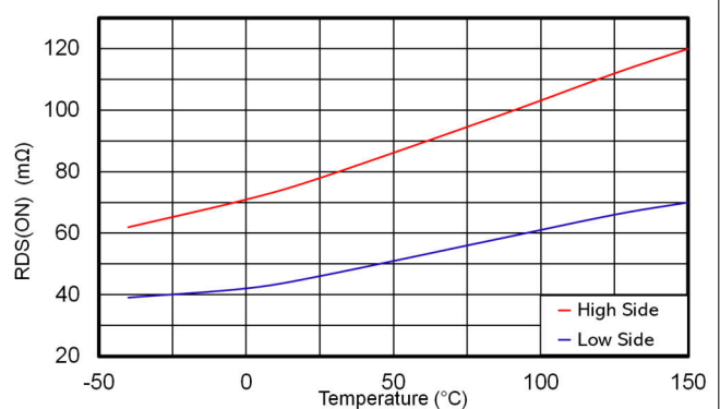
Figure 6-16. High Side and Low Side Switches R_{DS\_ON}
