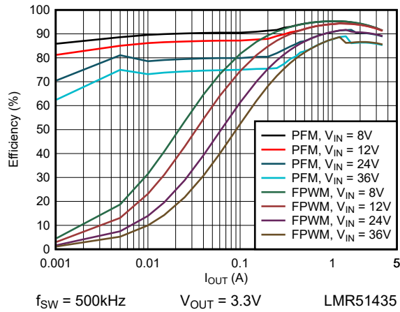
Figure 6-3. 3.3V Efficiency versus Load Current
