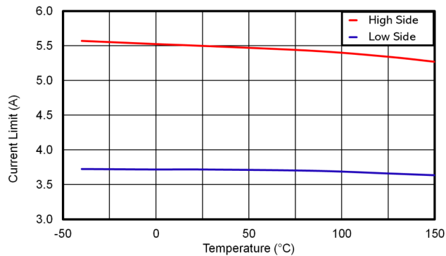
Figure 6-17. LMR51435 High Side and Low Side Current Limits
