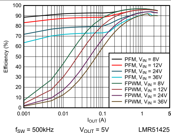
Figure 6-5. 5V Efficiency versus Load Current
