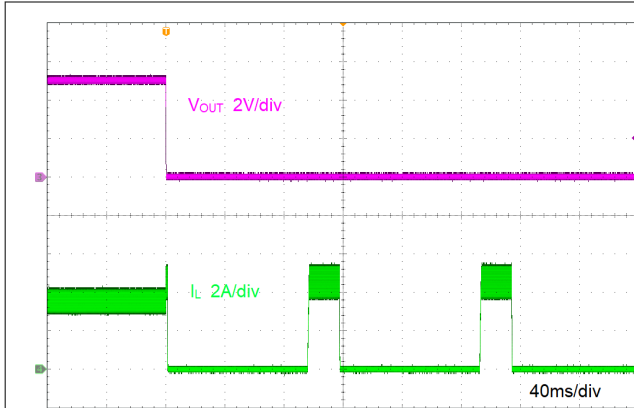
Figure 8-8. Short Protection
