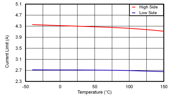
Figure 6-18. LMR51425 High Side and Low Side Current Limits
