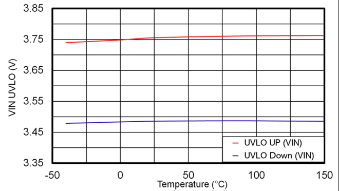
Figure 6-14. V_{IN} UVLO
