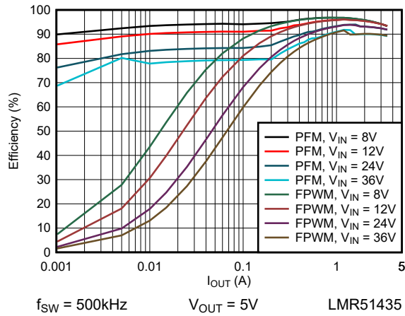
Figure 6-1. 5V Efficiency versus Load Current
