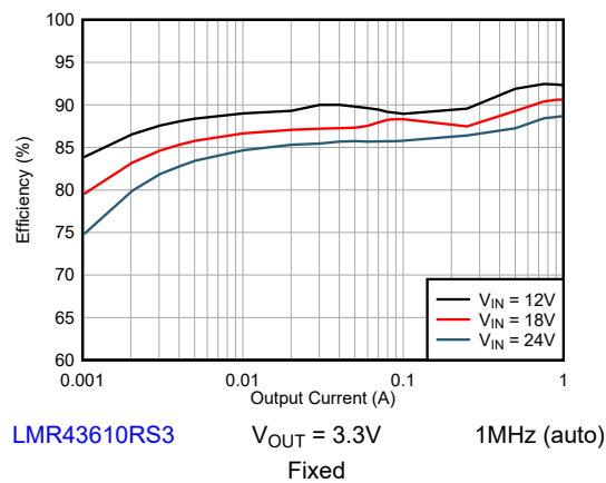
Figure 8-7. Efficiency
