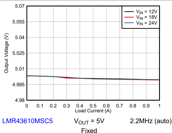
Figure 8-12. Line and Load Regulation
