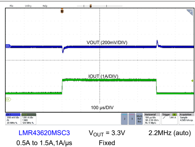
Figure 8-16. Load Transient
