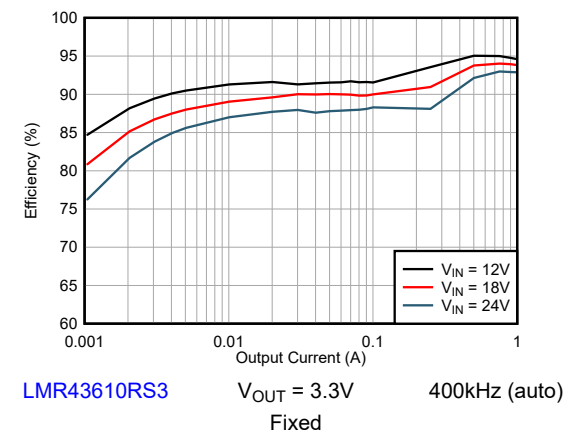
Figure 8-8. Efficiency
