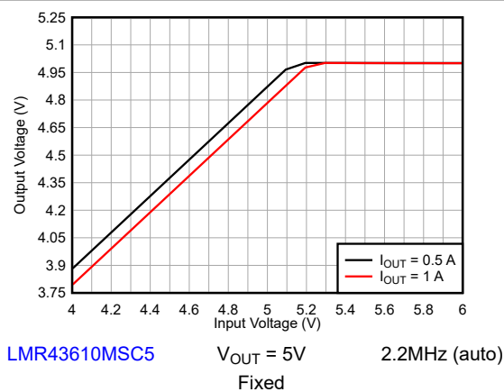
Figure 8-10. Dropout
