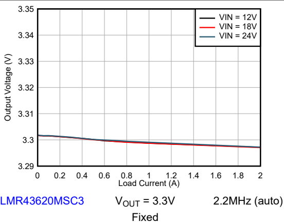
Figure 8-11. Line and Load Regulation
