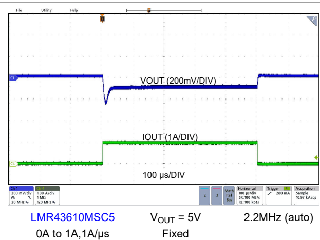
Figure 8-20. Load Transient
