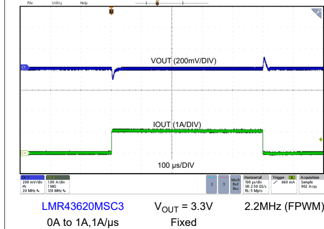
Figure 8-17. Load Transient
