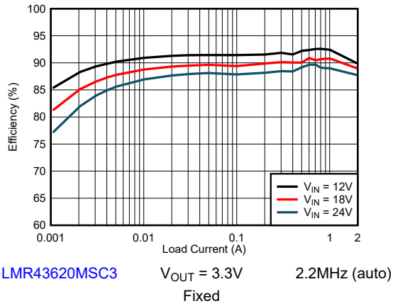
Figure 8-3. Efficiency
