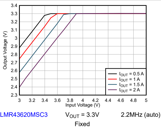
Figure 8-9. Dropout
