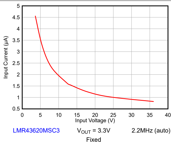
Figure 8-13. Input Switching Current vs. Input Voltage
