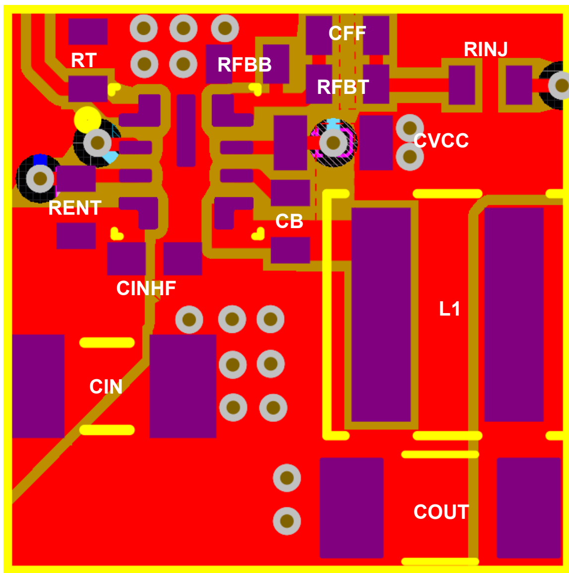
Figure 8-32. Example Layout
