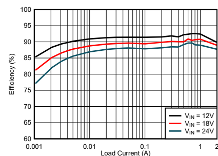
Efficiency: V OUT = 3.3V (Fixed), 2.2MHz
