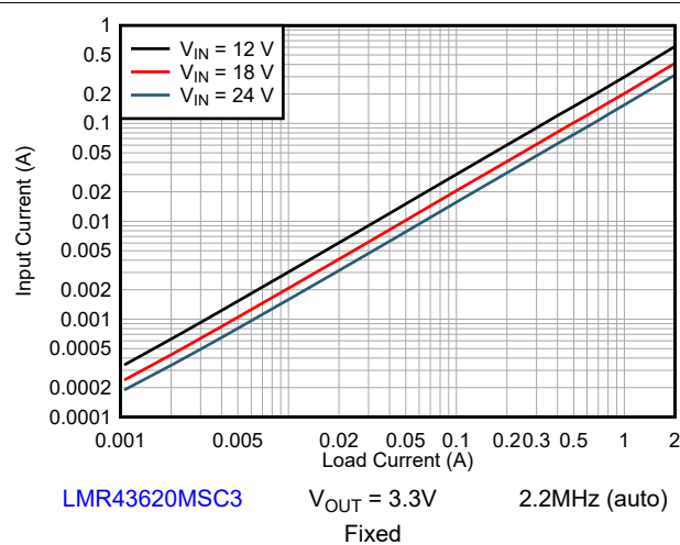
Figure 8-14. Input Current vs. Load Current
