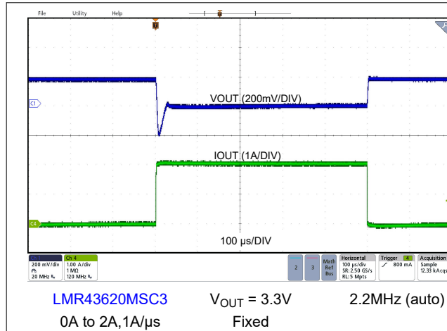
Figure 8-15. Load Transient
