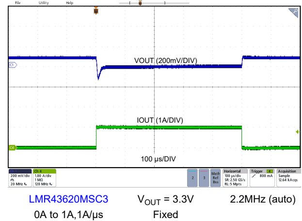
Figure 8-18. Load Transient
