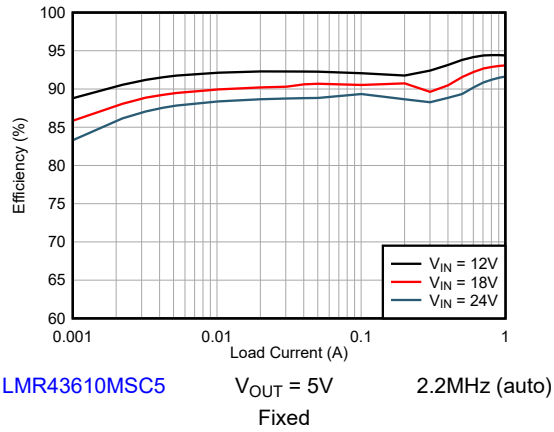
Figure 8-5. Efficiency
