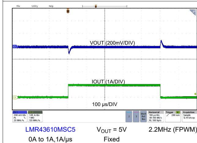
Figure 8-19. Load Transient
