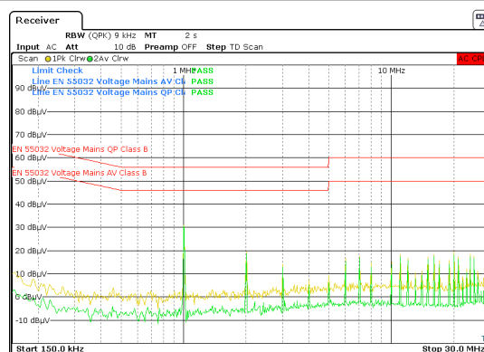
LMR43620MB5 Fixed V_{OUT} = 5\text{ V} V_{IN} = 24\text{ V} f_{SW} = 1\text{ MHz} I_{OUT} = 2\text{ A}
