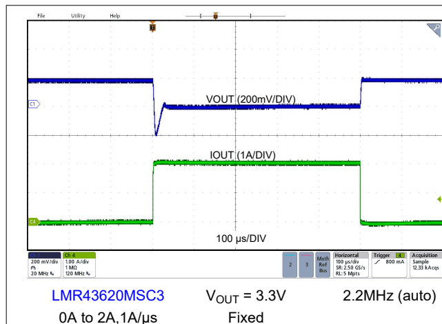
Figure 8-15. Load Transient
