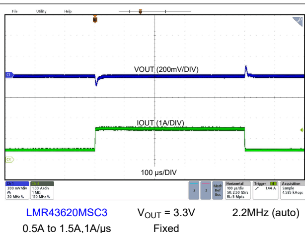
Figure 8-16. Load Transient
