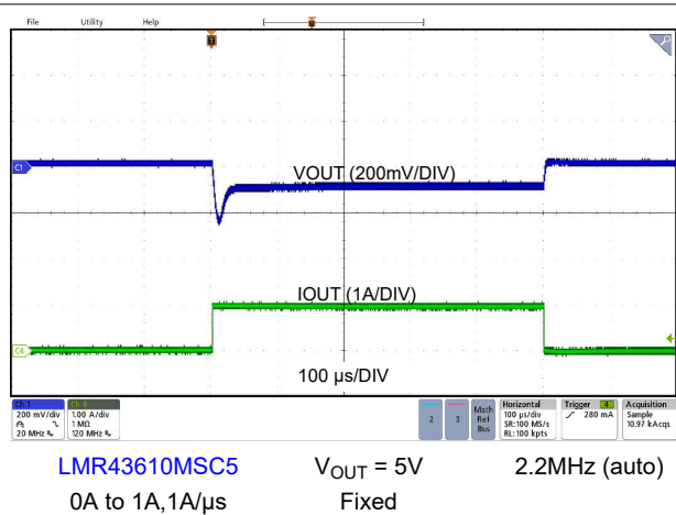
Figure 8-20. Load Transient
