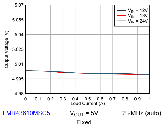
Figure 8-12. Line and Load Regulation
