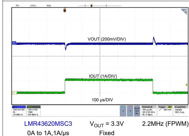
Figure 8-17. Load Transient
