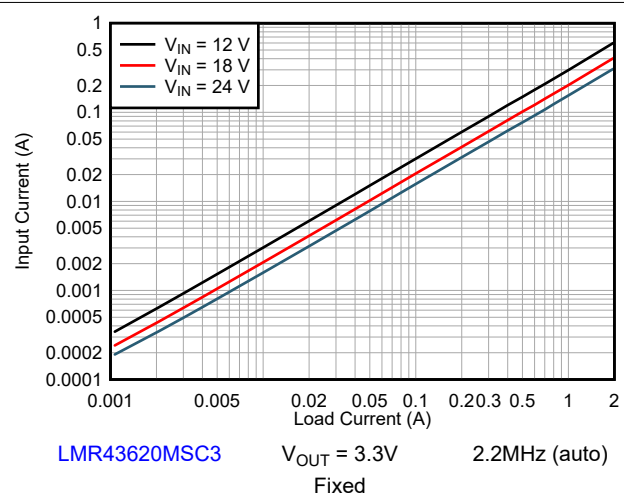
Figure 8-14. Input Current vs. Load Current
