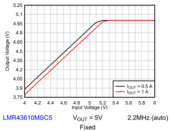
Figure 8-10. Dropout
