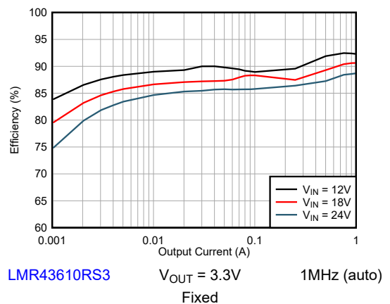
Figure 8-7. Efficiency
