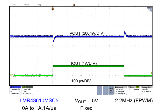
Figure 8-19. Load Transient
