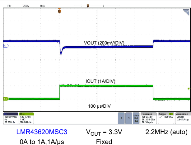
Figure 8-18. Load Transient
