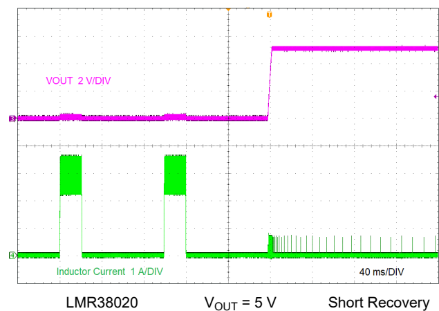
Figure 9-8. Short-Circuit Recovery
