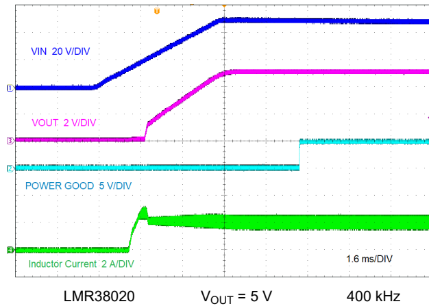
Figure 9-3. Start-Up by VIN
