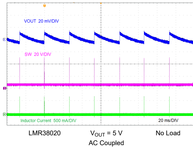
Figure 9-5. PFM Switching
