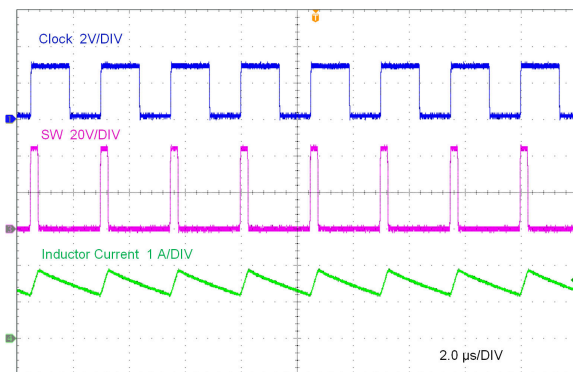
LMR38015-Q1 V_{OUT} = 5\text{ V} 400 kHz
