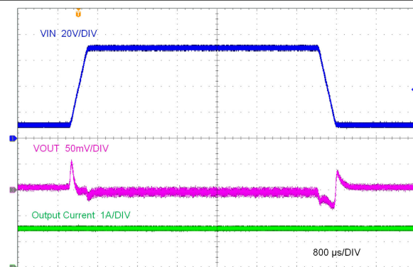
LMR38015-Q1 V_{OUT} = 5\text{ V} 400 kHz (AC Coupled) 10 V to 70 V at 200 V/ms
