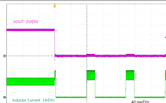
LMR38015-Q1 V_{OUT} = 5\text{ V} 1 A to Short
