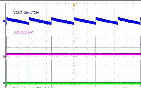
LMR38015-Q1 V_{OUT} = 5\text{ V} No Load
