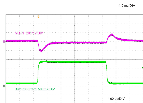
LMR38015-Q1 V_{OUT} = 5\text{ V} 400 kHz (AC Coupled) 150 mA to 1350 mA at 200 mA/μs
