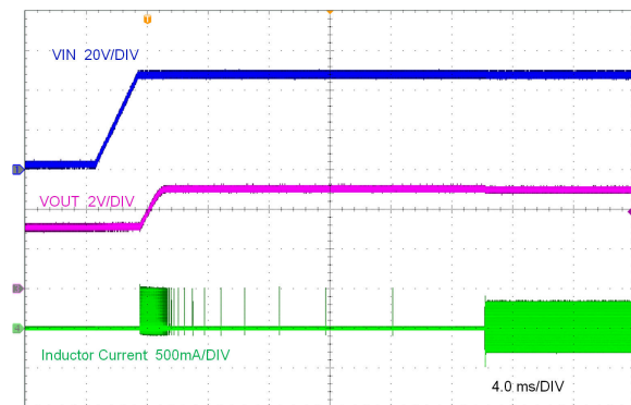
LMR38015-Q1 V_{OUT} = 5\text{ V} No Load Bias to 3 V
