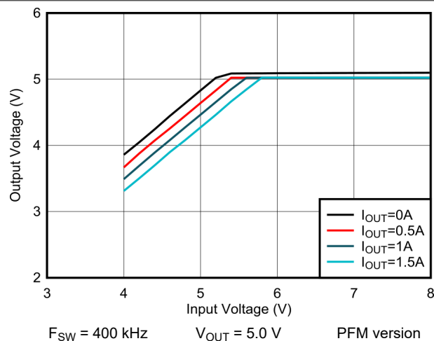
Figure 6-3. 5-V Dropout
