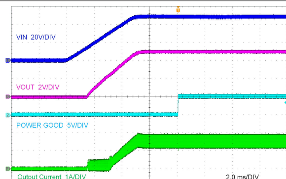
LMR38015-Q1 V_{OUT} = 5\text{ V} 400 kHz
