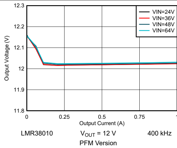
Figure 9-14. 12-V Load Regulation
