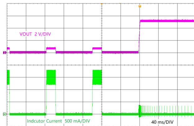
LMR38010 V_{OUT} = 5\text{ V} Short Recovery
