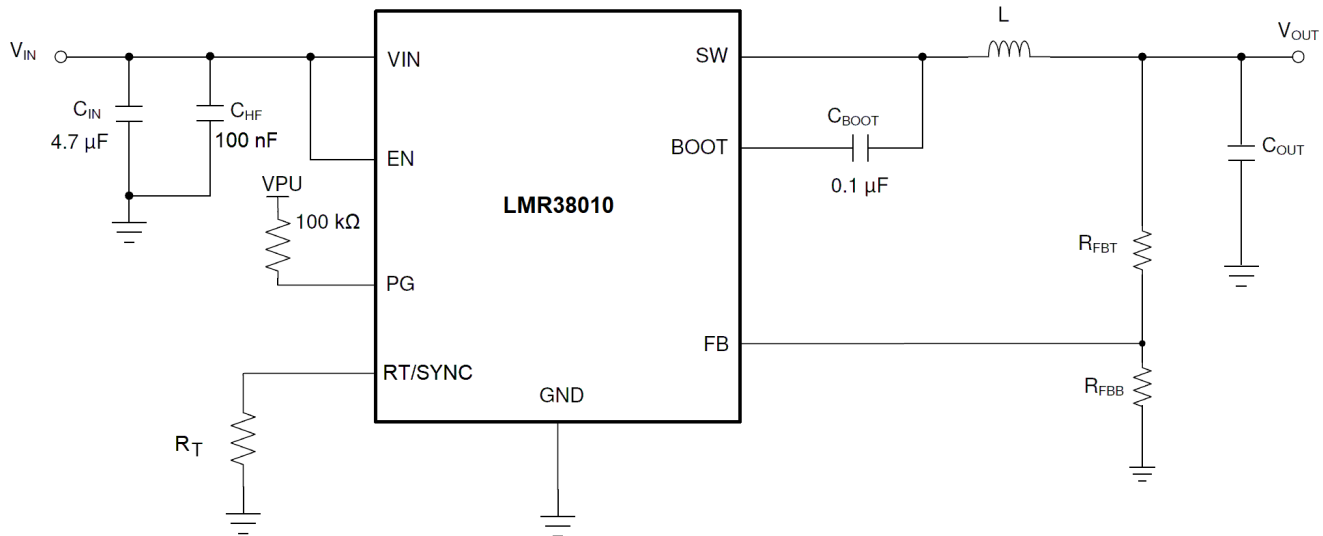
Figure 9-1. Example Application Circuit
