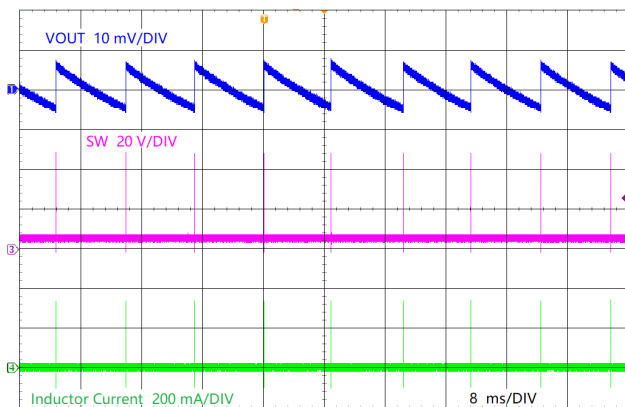
LMR38010 V_{OUT} = 5\text{ V} AC Coupled No Load
