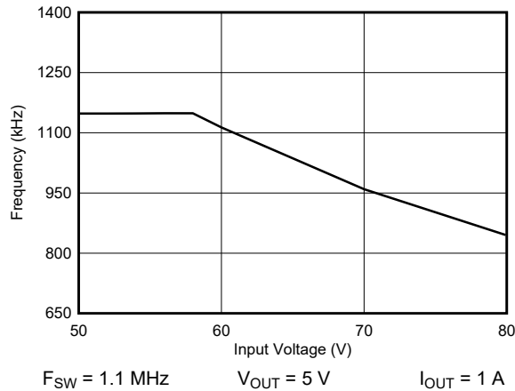
Figure 8-8. Typical Frequency Foldback at T ON_MIN
