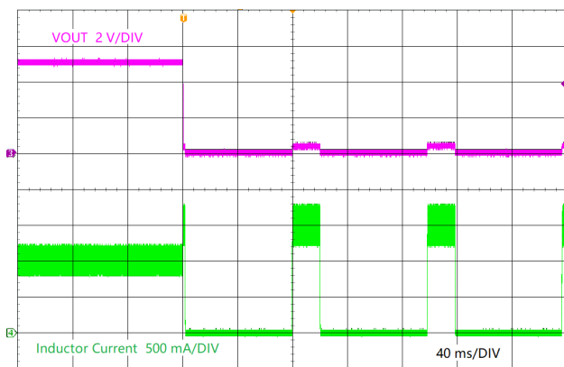
LMR38010 V_{OUT} = 5\text{ V} 1 A to Short
