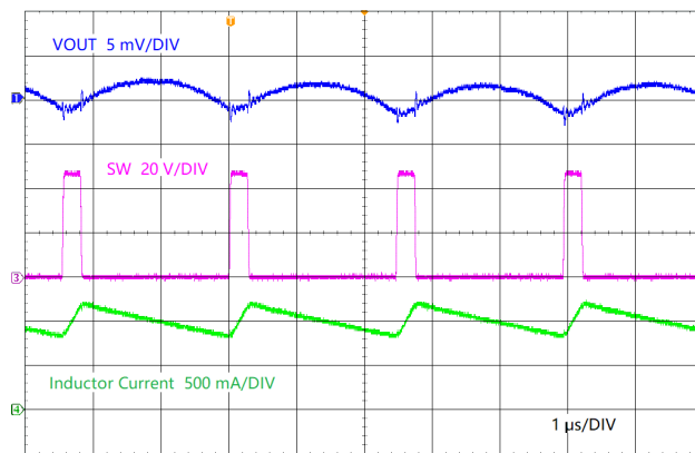
LMR38010 V_{OUT} = 5\text{ V} AC Coupled 400 kHz
