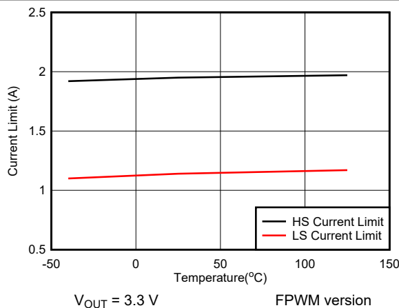
Figure 7-5. High-Side and Low-Side Current Limit vs Temperature
