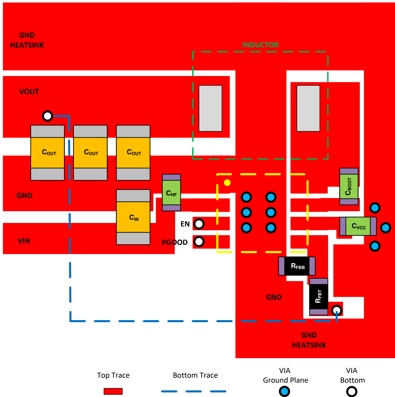
Figure 34. Example Layout
