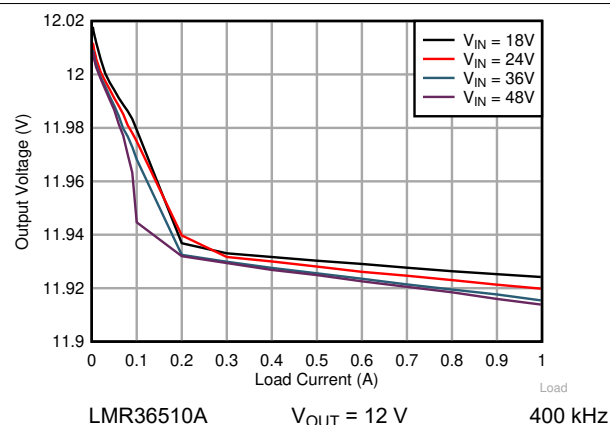
Figure 8-9. Load Regulation
