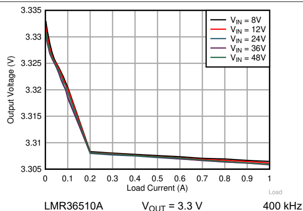
Figure 8-5. Load Regulation
