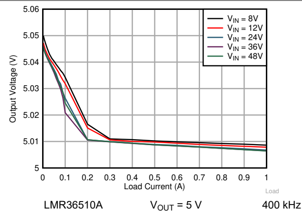
Figure 8-7. Load Regulation
