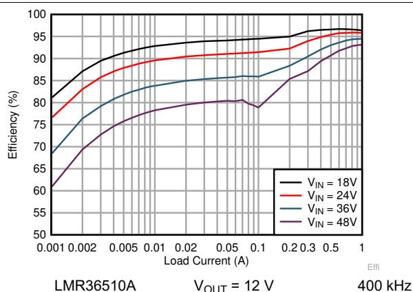
Figure 8-8. Efficiency
