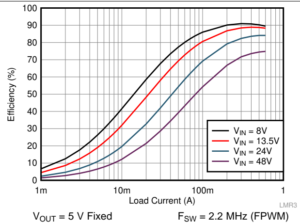
Figure 2. Efficiency 5-V Output, FPWM
