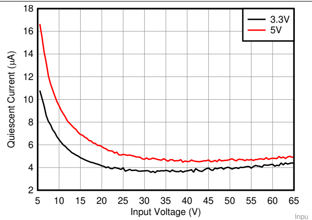
Figure 4. Typical Input Supply Current at No Load for Fixed 3.3-V and 5-V Output
