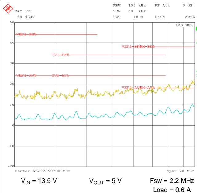
Figure 56. Typical CISPR 25 Conducted EMI 30MHz - 108MHz Yellow: Peak Detect, Blue = Average Detect
