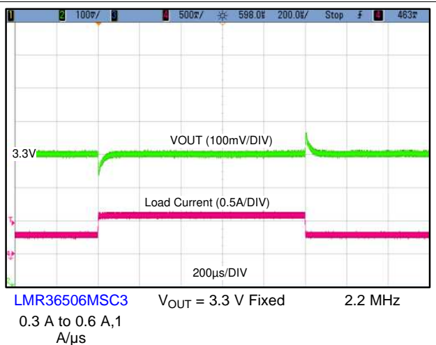
Figure 44. Load Transient
