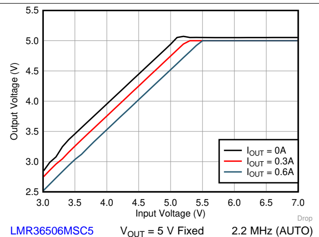
Figure 42. Dropout
