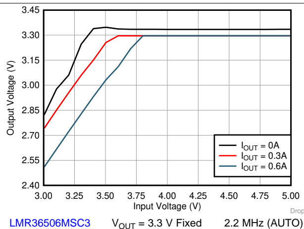
Figure 41. Dropout
