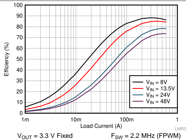
Figure 1. Efficiency 3.3-V Output, FPWM
