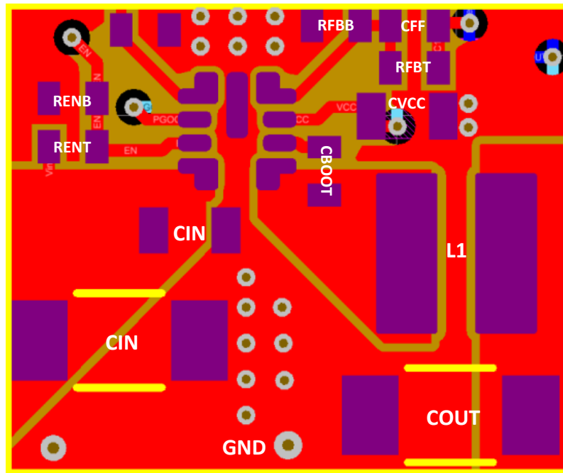
Figure 60. Example Layout
