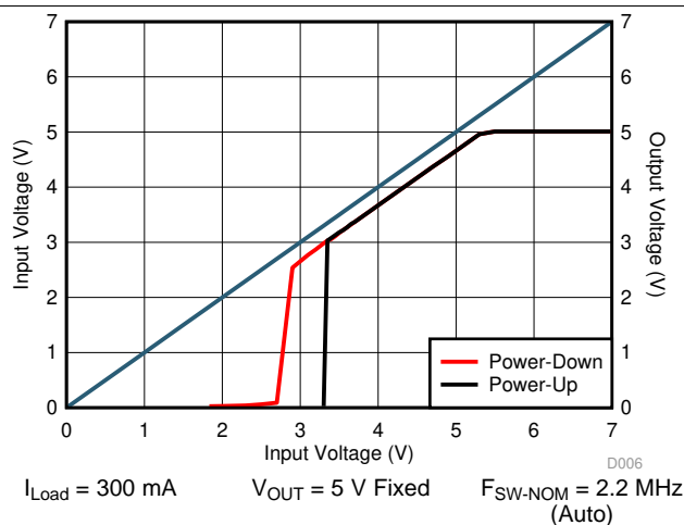
Figure 5. Dropout at Power-Up and Power-Down
