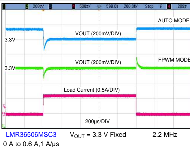
Figure 43. Load Transient
