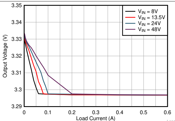
LMR36506RS3 V_{OUT} = 3.3 V Fixed 400 kHz (AUTO)
