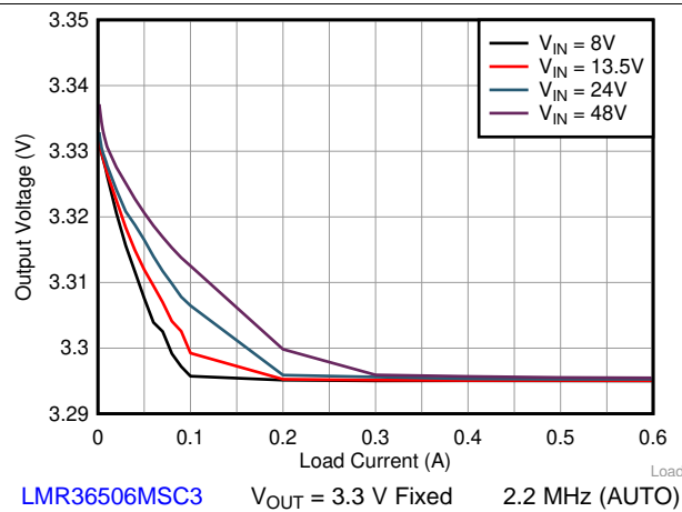
Figure 39. Line and Load Regulation
