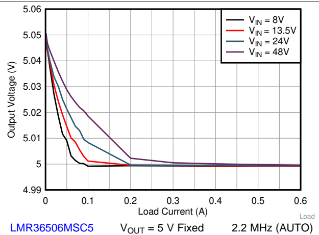
Figure 40. Line and Load Regulation
