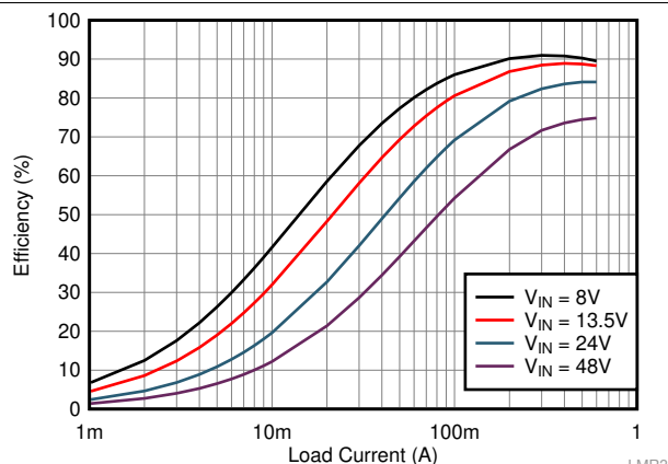
LMR36506MSC5 V_{OUT} = 5 V Fixed 2.2 MHz (FPWM)
