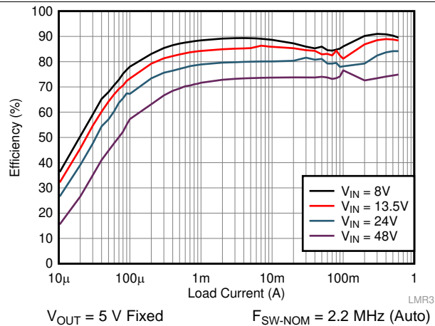
Figure 3. Efficiency 5-V Output, Auto Mode
