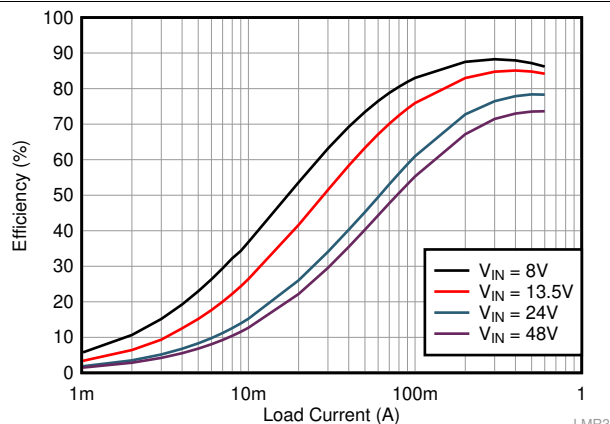
LMR36506MSC3 V_{OUT} = 3.3 V Fixed 2.2 MHz (FPWM)
