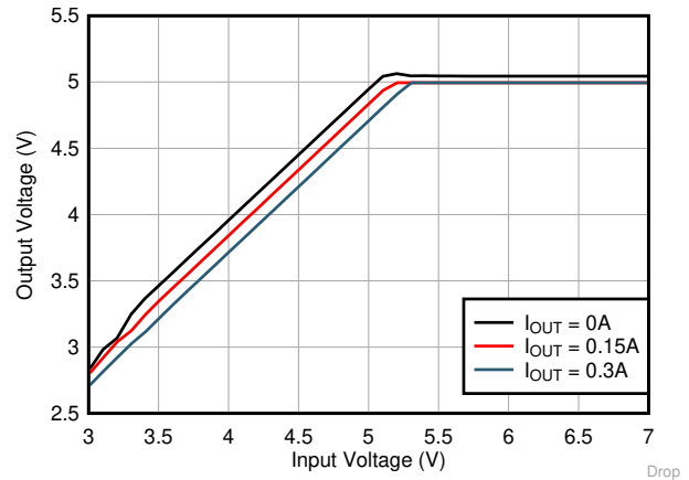
LMR36503MSC5 V_{OUT} = 5V Fixed 2.2 MHz (AUTO)
