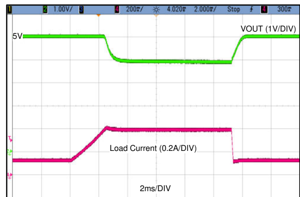
Figure 8-16. Overload Output Recovery
