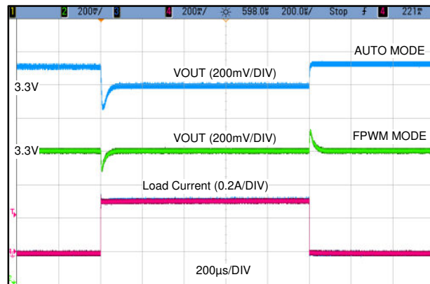
LMR36503MSC3 V_{OUT} = 3.3V Fixed 2.2 MHz 0 A to 0.3 A, 1 A/μs
