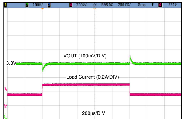
LMR36503MSC3 V_{OUT} = 3.3V Fixed 2.2 MHz 0.15 A to 0.3 A, 1 A/μs
