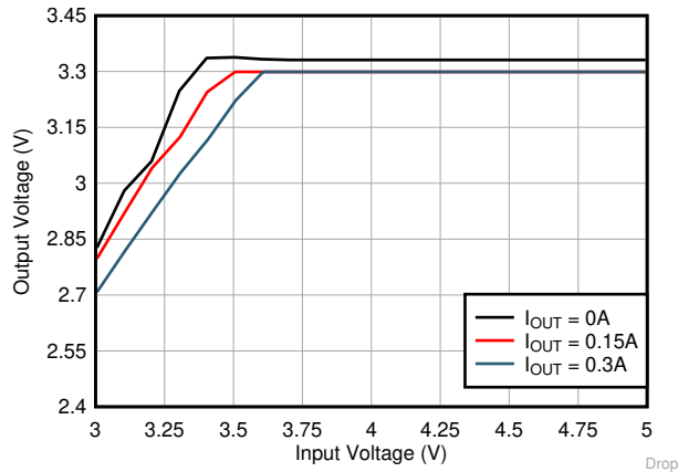
LMR36503MSC3 V_{OUT} = 3.3V Fixed 2.2 MHz (AUTO)
