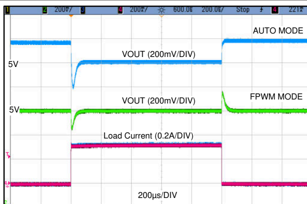
LMR36503MSC5 V_{OUT} = 5V Fixed 2.2 MHz 0 A to 0.3 A, 1 A/μs
