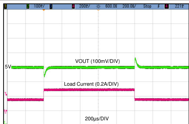
LMR36503MSC5 V_{OUT} = 5V Fixed 2.2 MHz 0.15 A to 0.3 A, 1 A/μs
