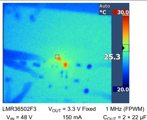
Figure 9-14. Thermal Image
