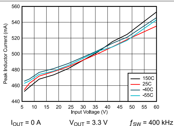
Figure 8-6. I_{PEAK-MIN}
