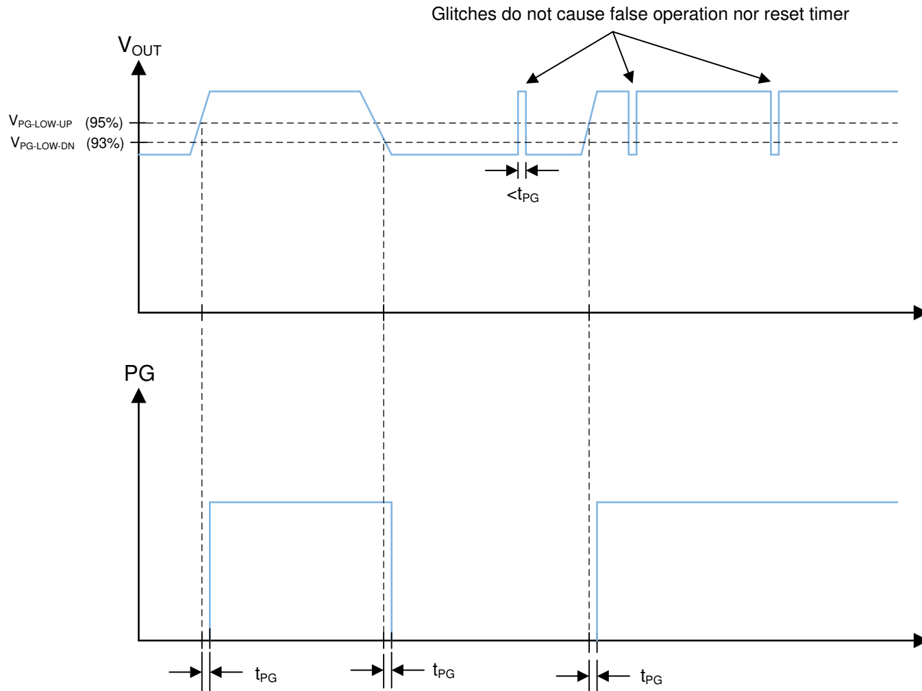
Figure 9. Power-Good-Timing Behavior
