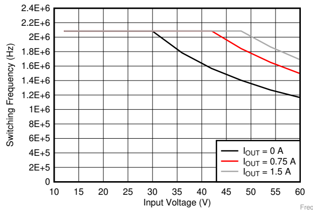
Figure 17. Switching Frequency vs Input Voltage VOUT = 5 V
