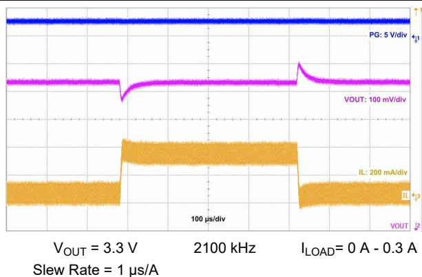
Figure 9-32. Load Transient
