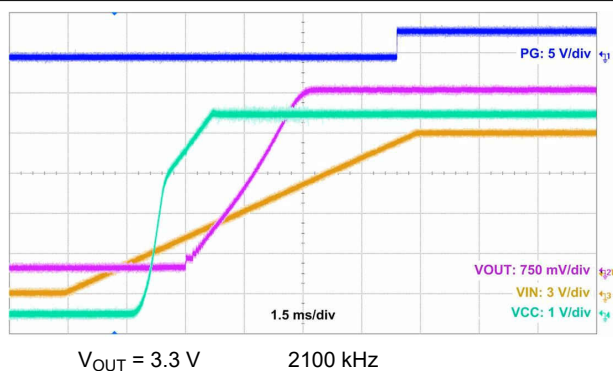
Figure 9-31. Start-Up Waveform
