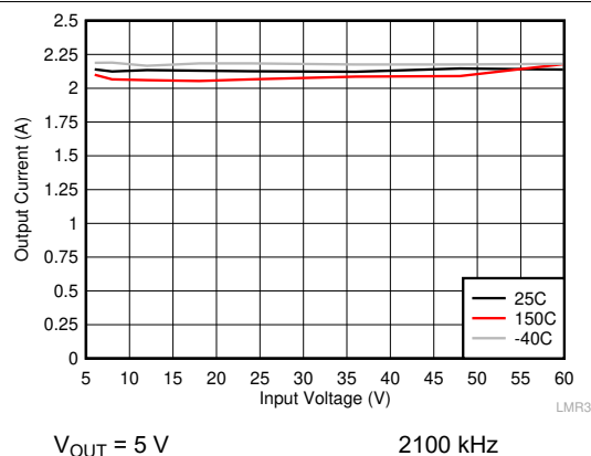
Figure 9-8. Load Current to Trigger Short Circuit
