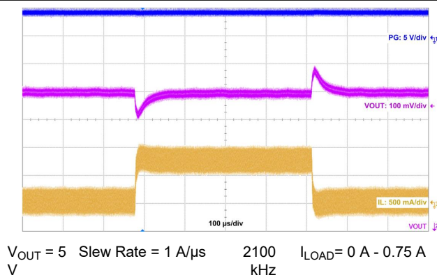
Figure 9-10. Load Transient Waveform
