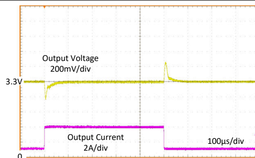
Figure 9-12. Load Transient
