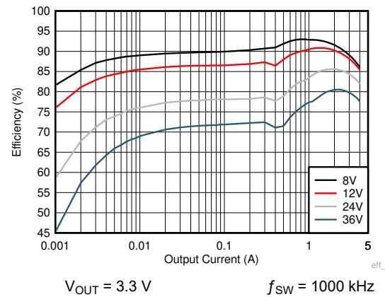
Figure 9-8. Efficiency
