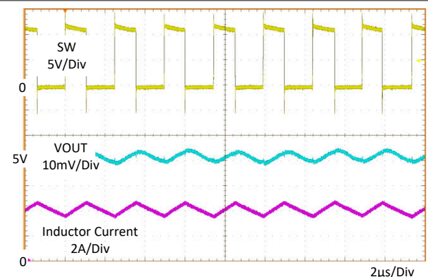
Figure 8-9. Typical PWM Switching Waveforms V_{IN} = 12\text{ V} , V_{OUT} = 5\text{ V} , I_{OUT} = 4\text{ A} , f_s = 400\text{ kHz}
