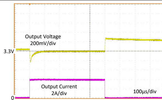
Figure 9-14. Load Transient
