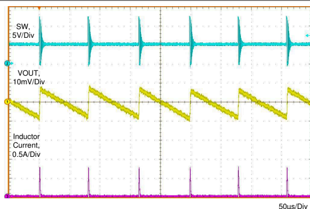
Figure 8-8. Typical PFM Switching Waveforms V_{IN} = 12\text{ V} , V_{OUT} = 5\text{ V} , I_{OUT} = 10\text{ mA}
