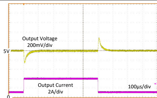
Figure 9-11. Load Transient
