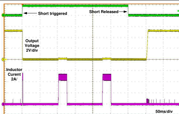
Figure 8-6. Short-Circuit Transient and Recovery V_{IN} = 12\text{ V} , V_{OUT} = 5\text{ V}
