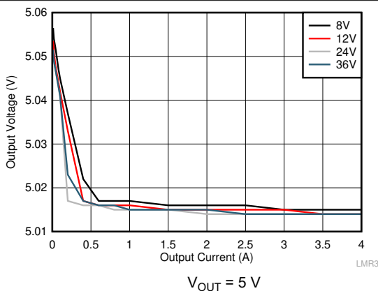
Figure 9-9. Line and Load Regulation
