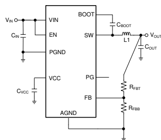
Simplified Schematic
