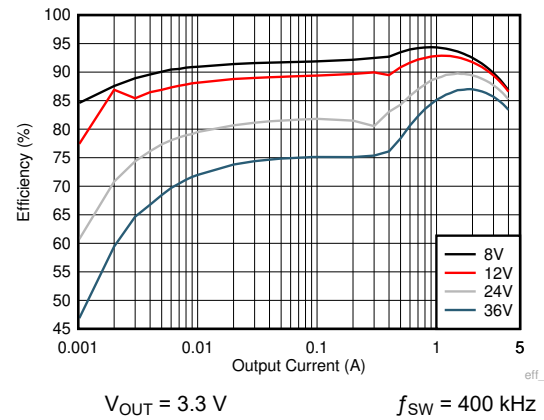
Figure 9-6. Efficiency
