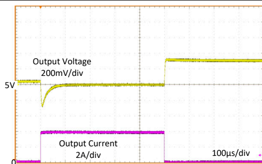
Figure 9-13. Load Transient
