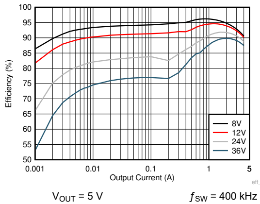
Figure 9-5. Efficiency
