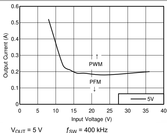
Figure 8-13. Mode Change Thresholds
