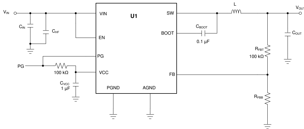
Figure 8-29. Circuit for Application Curves
