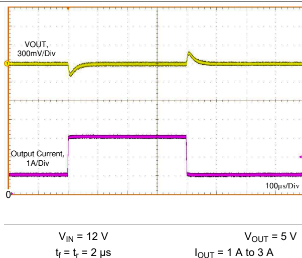
Figure 8-16. Load Transient
