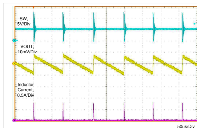
Figure 7-7. Typical PFM Switching Waveforms V_{IN} = 12\text{ V} , V_{OUT} = 5\text{ V} , I_{OUT} = 10\text{ mA}
