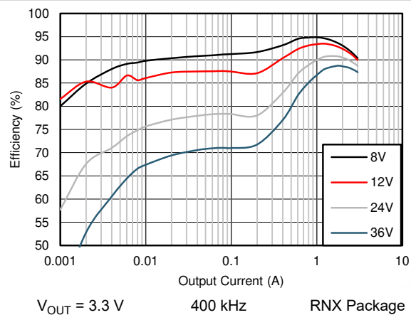
Figure 8-6. Efficiency
