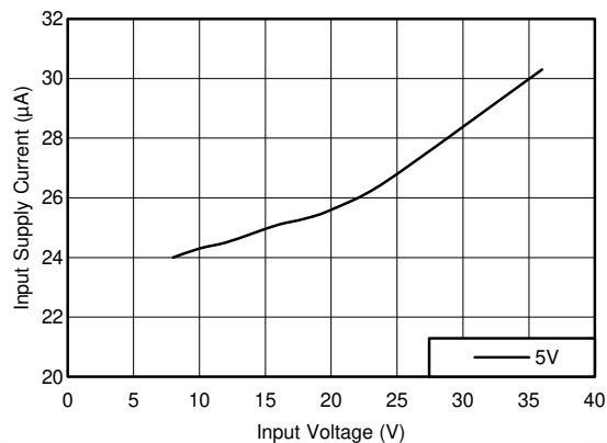
Figure 8-12. Input Supply Current
