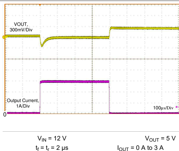
Figure 8-15. Load Transient
