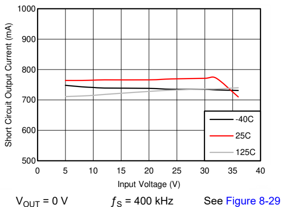
Figure 6-3. Short-Circuit Output Current
