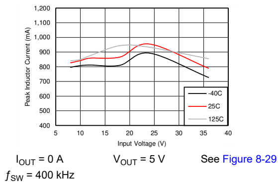
Figure 6-6. I_{PEAK-MIN}
