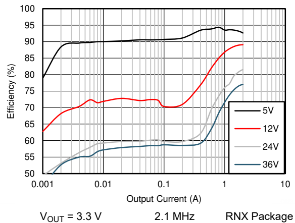
Figure 8-16. Efficiency
