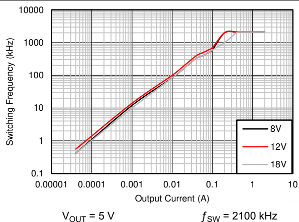
Figure 8-20. Switching Frequency versus Output Current
