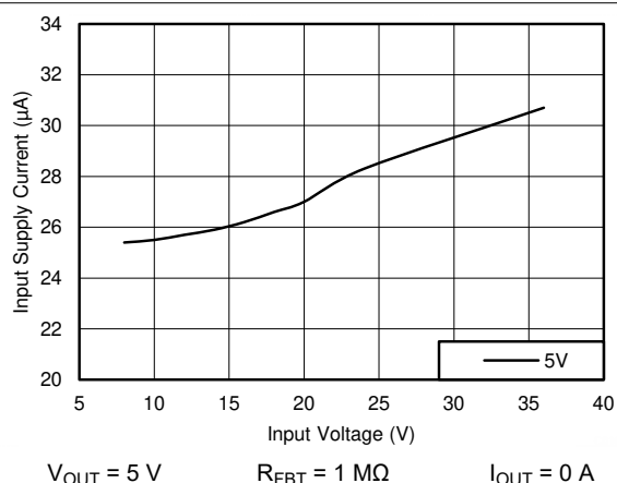
Figure 8-18. Input Supply Current
