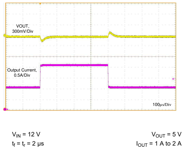
Figure 9-24. Load Transient
