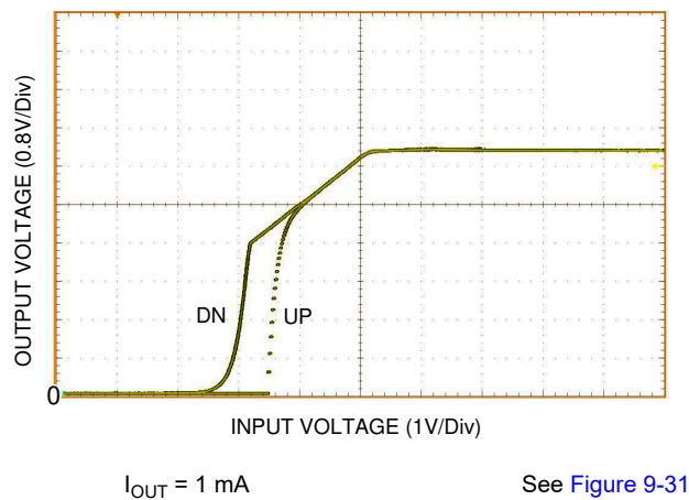
Figure 7-5. UVLO Thresholds
