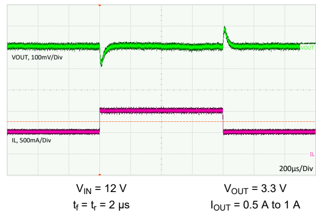
Figure 9-19. Load Transient
