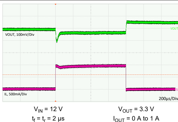
Figure 9-17. Load Transient
