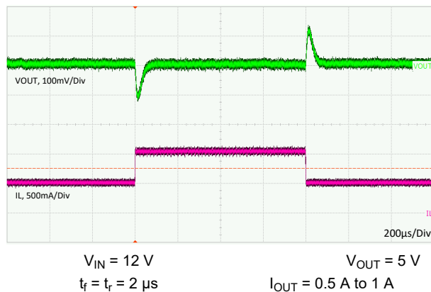
Figure 9-18. Load Transient
