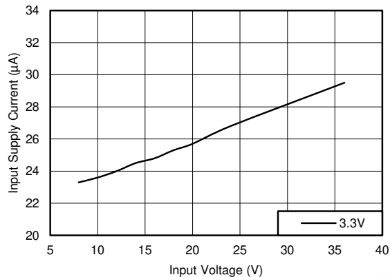
Figure 9-13. Input Supply Current
