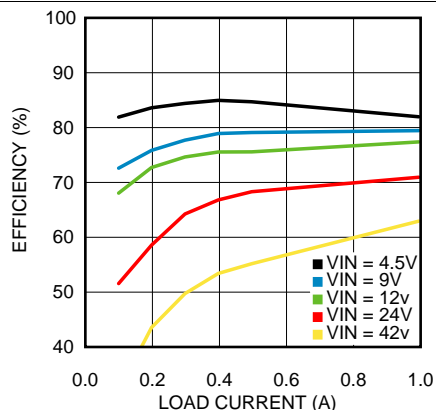
Figure 7. Efficiency vs Load Current
