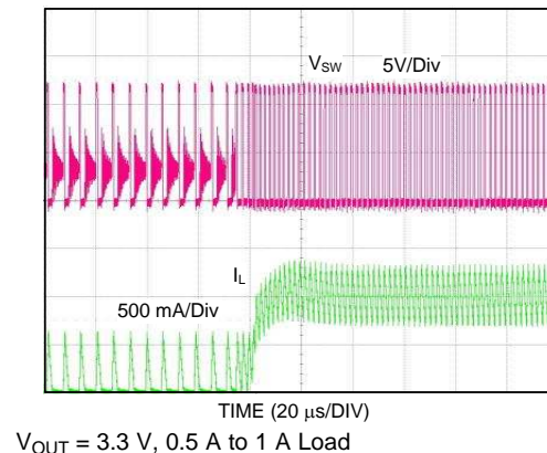
Figure 16. DCM to CCM Transition
