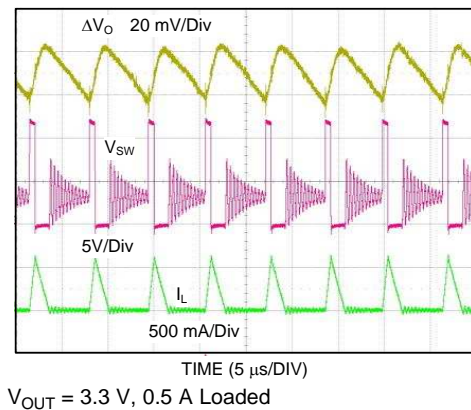
Figure 15. Discontinuous Mode Operation
