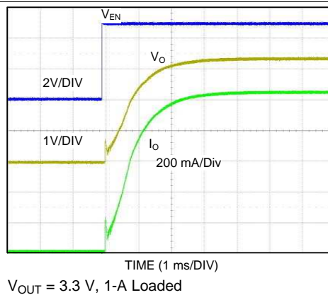
Figure 12. Enable Transient
