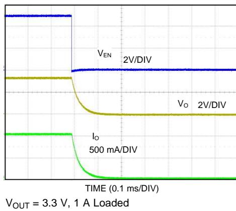
Figure 13. Shutdown Transient
