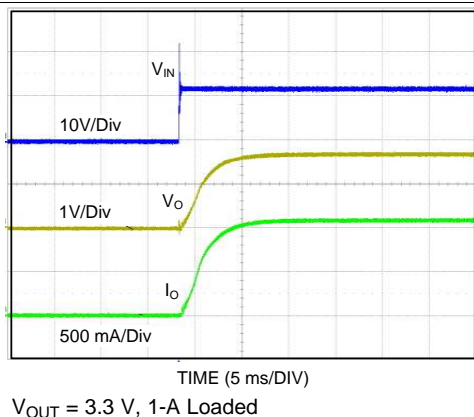
Figure 11. Power Up
