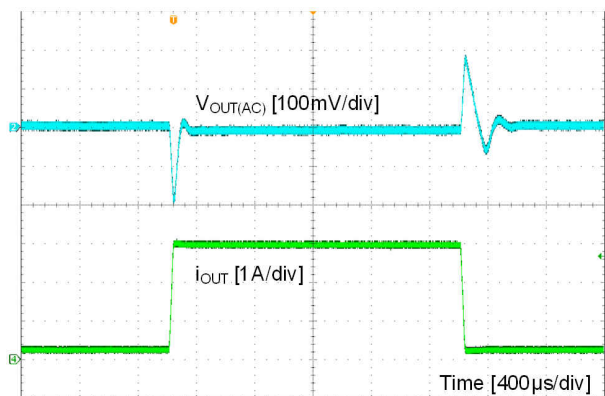
Figure 9-8. Load Transient
