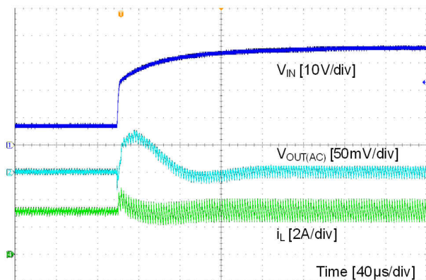
Figure 9-9. Line Transient
