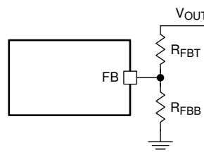
Figure 8-3. Output Voltage Setting
