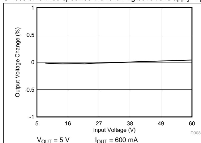
Figure 7. Line Regulation
