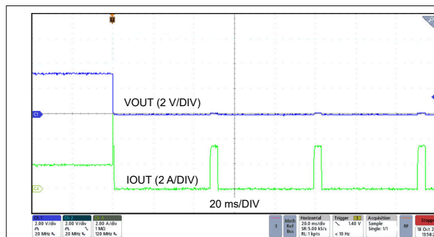
Figure 7-13. Hiccup Entry
