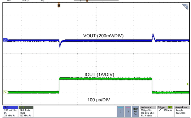
Figure 8-10. Load Transient
