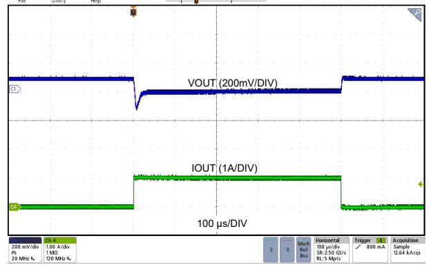
Figure 8-11. Load Transient
